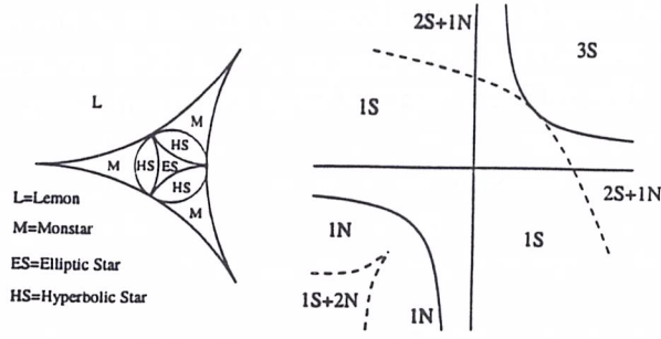
Figure 7: Partition of the set of cubics left, and of the (a, b) -plane right.
