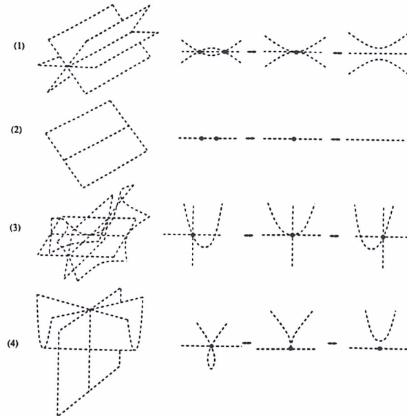
Figure 5: Changes on the A_3 -set at an umbilic: (1)-(2) a non-versal D_4 , (3) \alpha\beta = \mp 1 , (4) a D_5 -umbilic.
