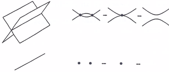
Figure 3: Changes on the parabolic set at a non-versal D_4 , real type top right, and imaginary type bottom right.
