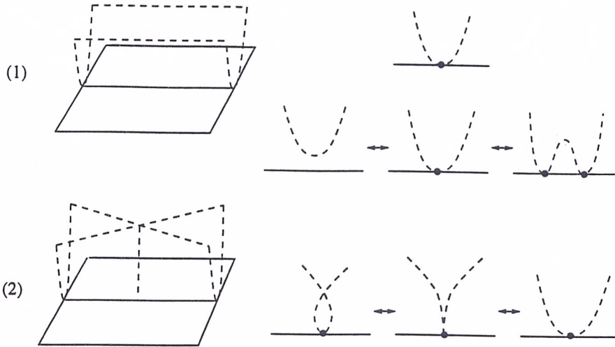
Figure 1: Changes on the A_3 -set (dashed) on a smooth parabolic curve (continuous).
