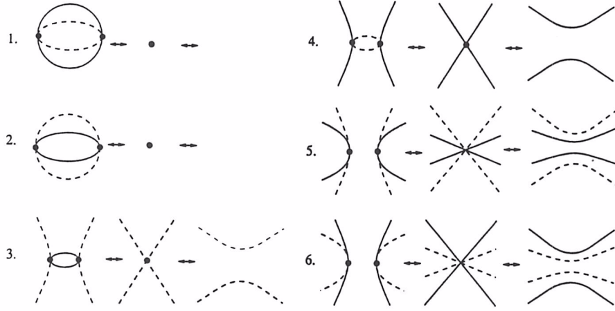
Figure 2: Morse transitions on the parabolic (continuous) and A_3 -sets (dashed).
