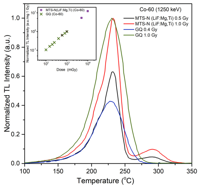
Fig. 5. The glow curve for MTS-N (LiF:Mg,Ti) (0.5 and 1.0 Gy) and Green quartz pellets (0.4 and 1.0 Gy) for gamma radiation. The TL Intensity was normalized with mass and TL response of 1 Gy. The upper inset shows the behavior of both dosimeters with dose. (For interpretation of the references to colour in this figure legend, the reader is referred to the Web version of this article.)
