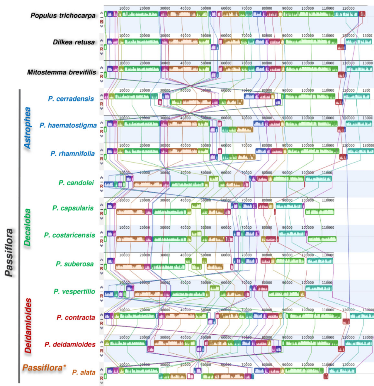
FIG. 2. —Synteny and structural rearrangements detected in the chloroplast genomes of 11 Passiflora species in addition to the Passifloraceae, Dilkea retusa and Mitostemma brevifilis , and the Salicaceae, Populus trichocarpa . Colored bars indicate syntenic blocks and connecting lines indicate the correspondence between blocks. *Species of the Passiflora subgenus obtained in this study share the same structure with Passiflora alata .
