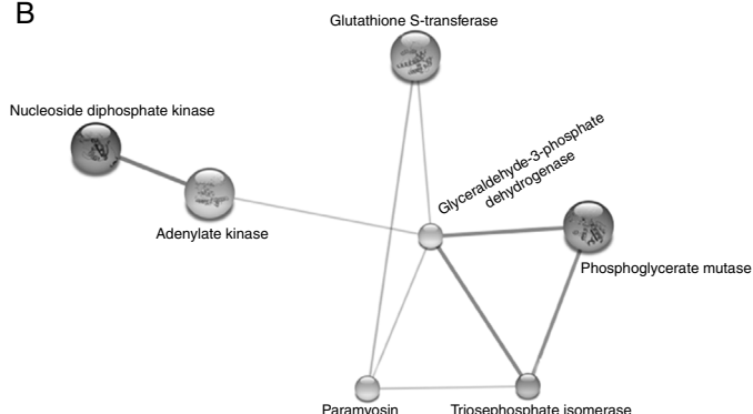
Fig. 3. Network of interactions from Schistosoma mansoni proteins affected by exposure to DNH. Identified S. mansoni proteins were matched to S. japonicum on STRING database v9.05. (A) Network of interactions on Cluster of orthologous groups/Eukaryotic orthologous groups (COG/KOG) mode. (B) Network of interactions on protein mode; nucleoside diphosphate kinase, adenylate kinase, glutathione S-transferase, glyceraldehyde-3-phosphate dehydrogenase, paramyosin, triosephosphate isomerase, phosphoglycerate mutase.
