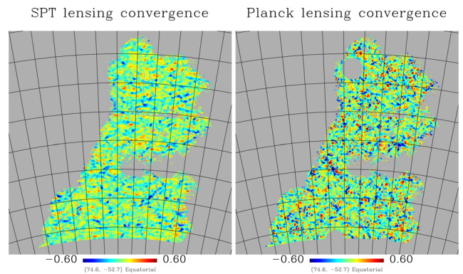
Figure 3. Maps of the CMB lensing convergence in the SPT-E field for SPT (left) and Planck (right), pixelated on the HEALPIX N_{\text{side}} = 2048 scheme (pixel side: 1.7 arcmin) in Equatorial coordinates, smoothed on angular scales of 10 arcmin to improve visualization. The grid lines are 2.5 apart. Grey areas indicate masked data. The DES mask has been applied for clarity, but we do not impose it on the CMB data in our cross-correlation estimation. The Planck lensing map also includes the Planck lensing mask. Planck shows higher amplitude variations, but this is due to higher noise caused by the lower spatial resolution of its map.
