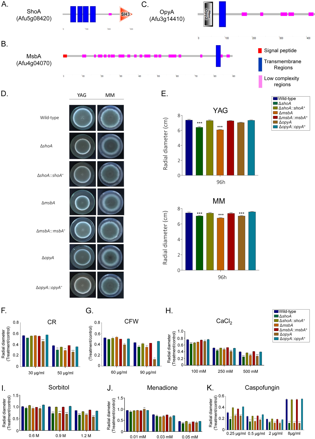
FIG 2 A. fumigatus ShoA, MsbA, and OpyA. (A to C) Protein organization of A. fumigatus ShoA (A), MsbA (B), and OpyA (C). (D to J) Growth phenotypes of the wild-type strain and the \Delta shoA , \Delta msbA , \Delta opyA , \Delta shoA::shoA^+ , \Delta msbA::msbA^+ , and \Delta opyA::opyA^+ mutants. The strains were (Continued on next page)
