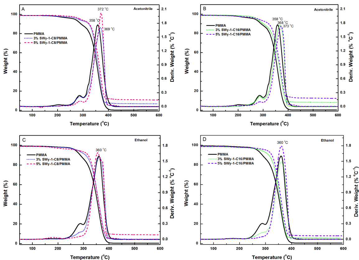
Figure 1. (a) and (b) TGA and DTG curves for PMMA and nanocomposites synthesized in acetonitrile; (c) and (d) PMMA and nanocomposites synthesized in ethanol.
