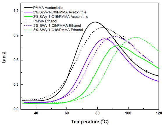
Figure 3. Temperature dependence of \tan \delta for PMMA and nanocomposites synthesized in acetonitrile and ethanol.
