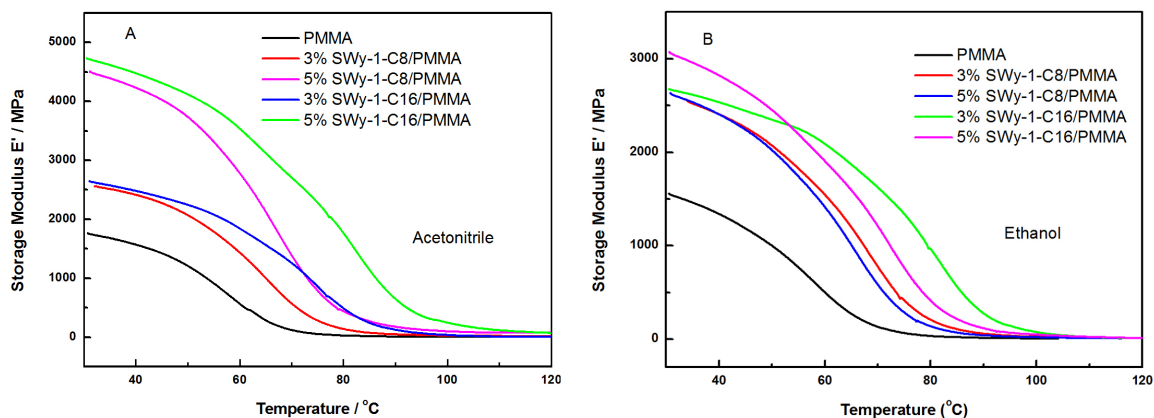
Figure 2. Temperature dependence of storage modulus ( E' ) of PMMA and nanocomposites synthesized in acetonitrile (a) and synthesized in ethanol (b).
