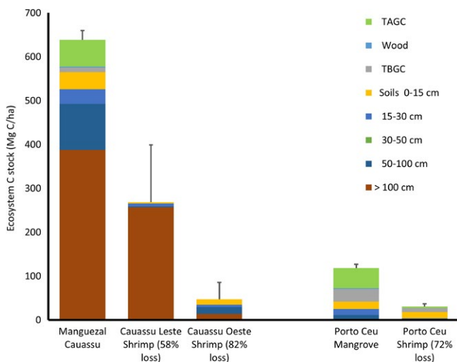
FIGURE 5 Ecosystem carbon stocks (Mg C/ha) of paired mangroves with adjacent shrimp ponds (TAGC = total above ground carbon pool and TBGC = total below ground plant carbon pool). The Manguelal Cauassú site was paired with two adjacent shrimp ponds (the Cauassú Leste and Oeste shrimp ponds) in the Rio Acaraú Estuary. The Porto Céu mangrove was adjacent to the Port Céu Shrimp pond in the Rio Jaguaribe Estuary. Vertical bars are one standard error of the mean total ecosystem carbon stock
