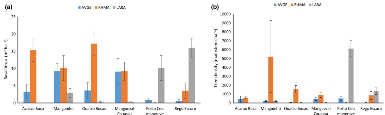
FIGURE 2 (a) The basal area ( \text{m}^2/\text{ha} ) and (b) density (main stems/ha) of mangroves sampled in Ceará, Brazil (AVGE = Avicennia germinans , RHMA = Rhizophora mangle , and LARA = Laguncularia racemosa ). Vertical bars represent \pm one standard error
