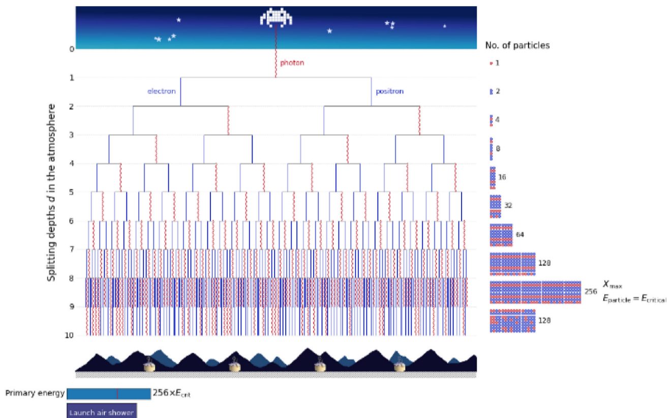
Fig. 8 Toy model for the development of an electromagnetic cascade in the atmosphere
