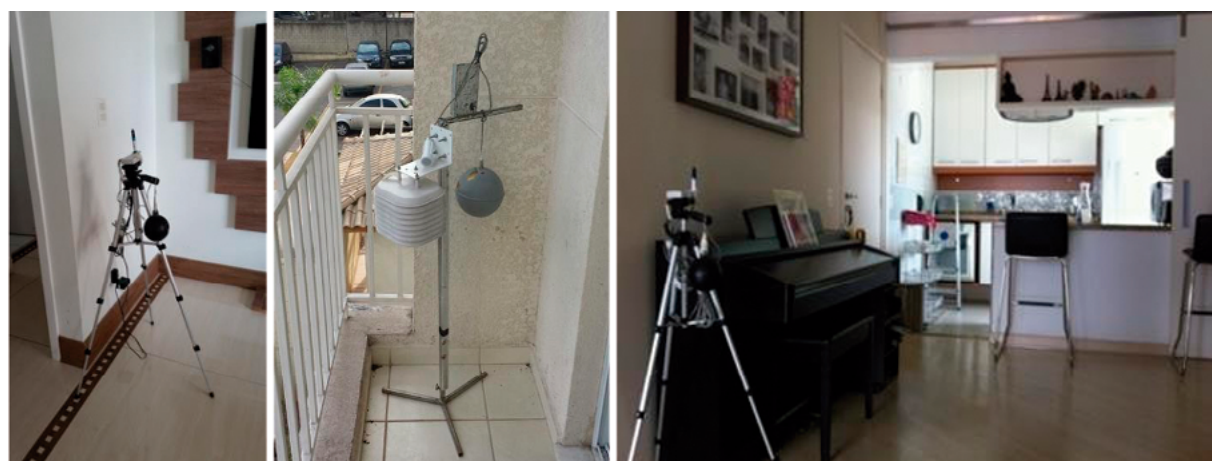
Figure 3. Indoor measurements in apartment buildings
