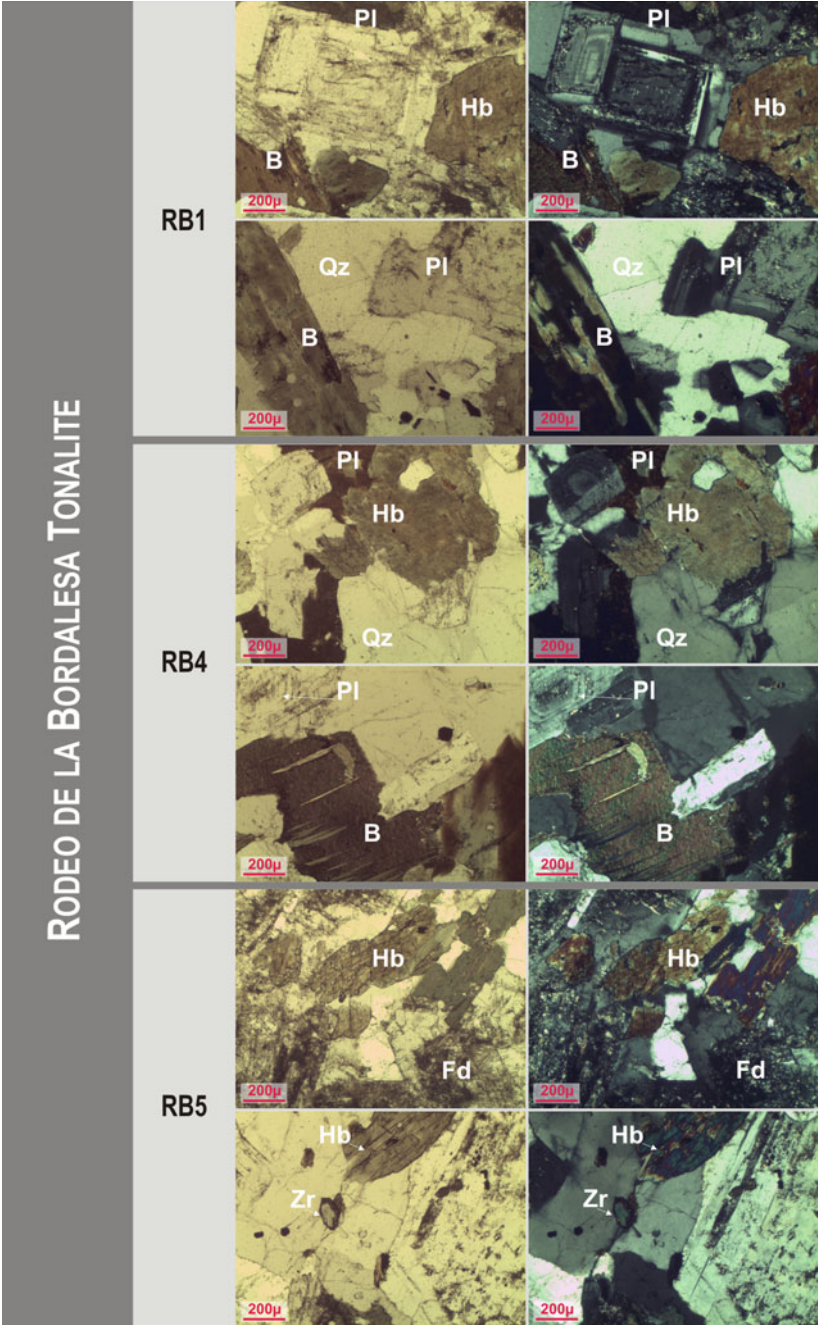
Fig. 4 Photomicrographs of the Rodeo de la Bordalessa tonalite samples showing equigranular texture. Pl zoned plagioclase; Hb hornblende; Qz quartz; Fd K-feldspar; B biotite, Zr zircon
