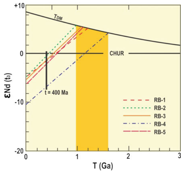
Fig. 11 The \epsilon_{\text{Nd}} evolution diagram of samples at t = 400\text{ Ma}
