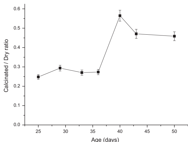
Fig. 3. Ratio of calcinated to dry weights as a function of the animals' age. The lines are only to guide the eyes.
