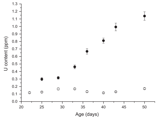
Fig. 1. Full circles: concentration of uranium in the femora of Wistar rats doped with uranyl nitrate expressed in parts per million (ppm), which is equivalent to \mu\text{g/g} , as function of the age. Open circles: the same as before for the control animals (fed with commercially available ration). See text for more details.
