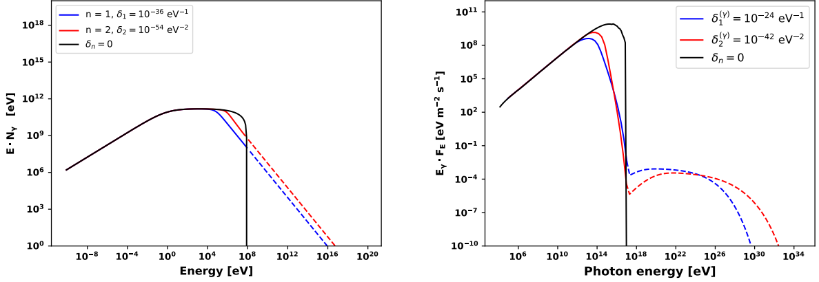
(a) Energy spectrum of photons emitted via sync. when sync. is the dominant loss process.
