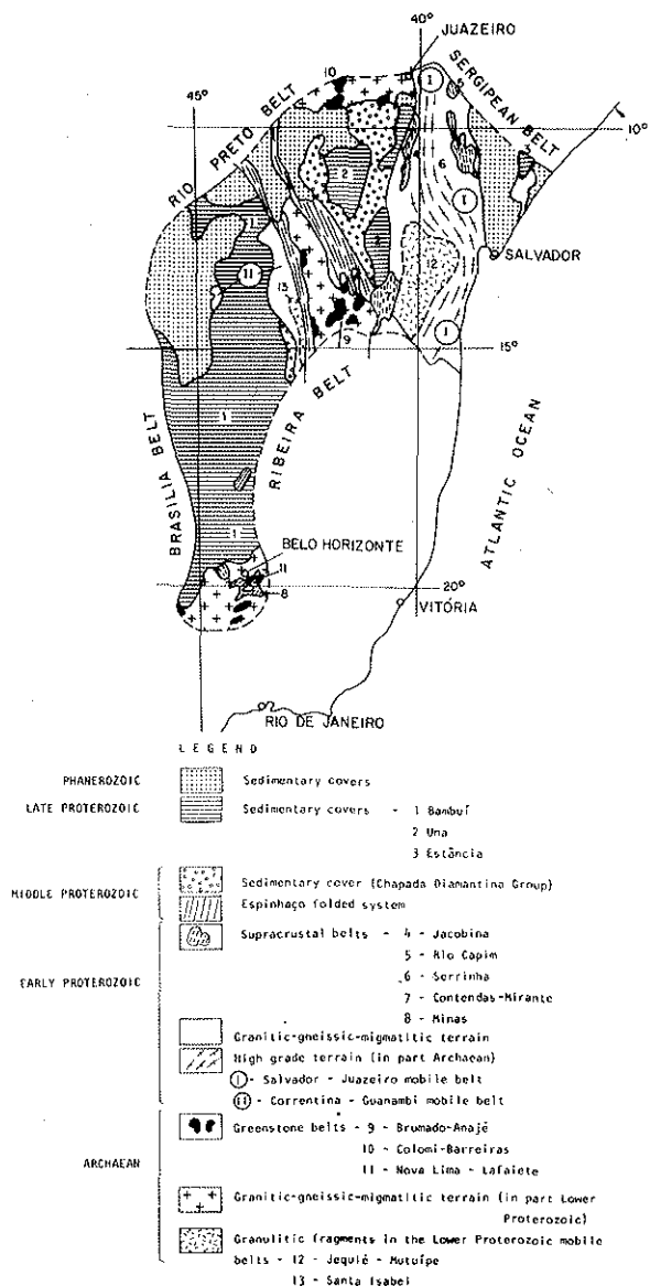
Figure 3 - The São Francisco craton
