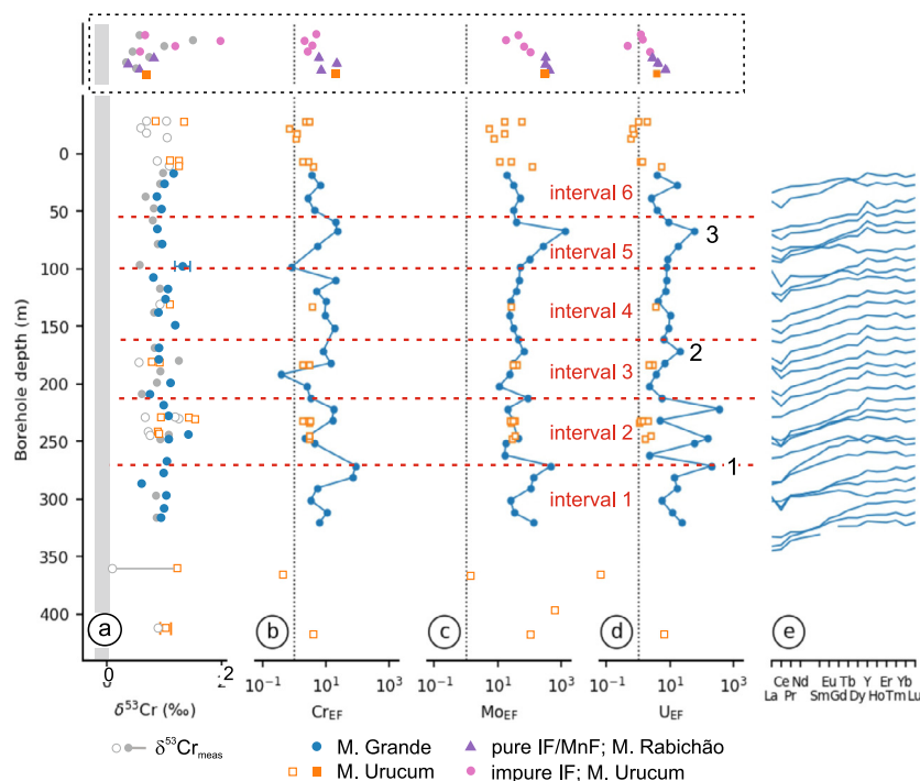
Fig. 10. Stratigraphic variation of \delta^{53}Cr_{auth} values, redox sensitive element EFs and PAAS normalized REY patterns. Bore hole depths correspond to those in Fig. 5, which contains the respective units and lithologies: (a) \delta^{53}Cr_{auth} blue filled circles are hematite mesoband samples from this study plotted with corresponding \delta^{53}Cr_{meas} filled grey circles (b) Cr_{EF} ; (c) Mo_{EF} ; (d) U_{EF} ; (e) Shale normalized REY patterns (Taylor and McLennan, 1985), Lu centered on sample depth. Open symbols (orange squares) indicate surface sample data from (Frei et al., 2017), plotted at approximate stratigraphic level. Samples without stratigraphic relation, analyzed for Cr isotope compositions herein, are plotted in the insert above (symbols as in Fig. 5). (For interpretation of the references to colour in this figure legend, the reader is referred to the web version of this article.)
