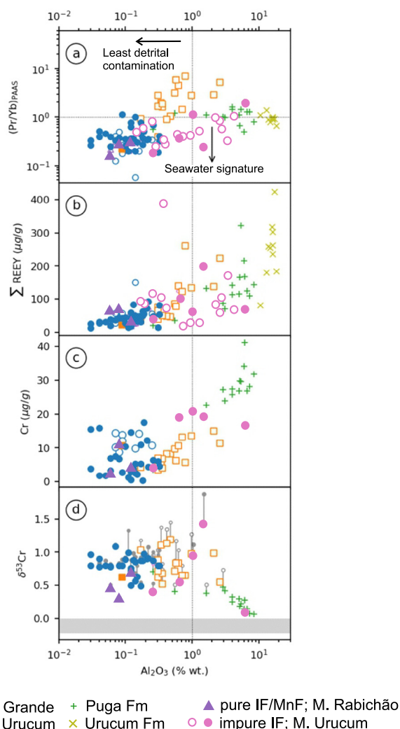
Fig. 12. Detrital influence (represented by \text{Al}_2\text{O}_3 ) on REY, Cr and \delta^{53}\text{Cr} values in IF. (a) (\text{Pr}/\text{Yb})_{\text{PAAS}} shows no significant correlation with \text{Al}_2\text{O}_3 , but there is a clear distinctive clustering of IFs from M. Grande analyzed herein (blue filled circles) from surface sample IFs at M. Urucum (empty orange squares; data from (Frei et al., 2017)). This discrepancy is attributed to the effects of supergene alteration of the surface samples on the REY pattern (see text for details). (b) Correlation between total REE + Y concentration and \text{Al}_2\text{O}_3 . The flat distribution depicted by the M. Grande samples studied herein (blue filled circles) in this diagram depicts that REEs are only weakly controlled by detrital siliciclastic components. (c) Lack of a systematic relationship between Cr concentration and \text{Al}_2\text{O}_3 in the IF samples from M. Grande (studied herein, blue filled circles) and in the surface IF samples from M. Urucum (empty orange squares; data from (Frei et al., 2017)) attests for a dominance of an authigenic Cr fraction in these IFs. In contrast, a significant correlation of Cr with \text{Al}_2\text{O}_3 exists in iron rich shale from the Puga Formation and in impure IFs from M. Urucum. (d) Lack of correlation of raw (i.e., measured, uncorrected for Cr contribution from detrital siliciclastics) \delta^{53}\text{Cr} in IF samples with below ca. 1 wt. \text{Al}_2\text{O}_3 attests to a predominantly authigenic Cr isotope signature in these IFs. In contrast, samples from the Puga Formation show a clear trend towards unfractionated \delta^{53}\text{Cr} values with rising \text{Al}_2\text{O}_3 . Measured (i.e., uncorrected for contamination of Cr by detrital siliciclastics) \delta^{53}\text{Cr} are shown with gray open and closed circles that are connected to respective symbols marking authigenic compositions. Filled symbols are from this study. Open symbols and crosses indicate data from (Angerer et al., 2016), (Viehmann et al., 2016) and (Frei et al., 2017). The gray shaded band marks the igneous silicate Earth reservoir defined by (Schoenberg et al., 2008). (For interpretation of the references to colour in this figure legend, the reader is referred to the web version of this article.)
