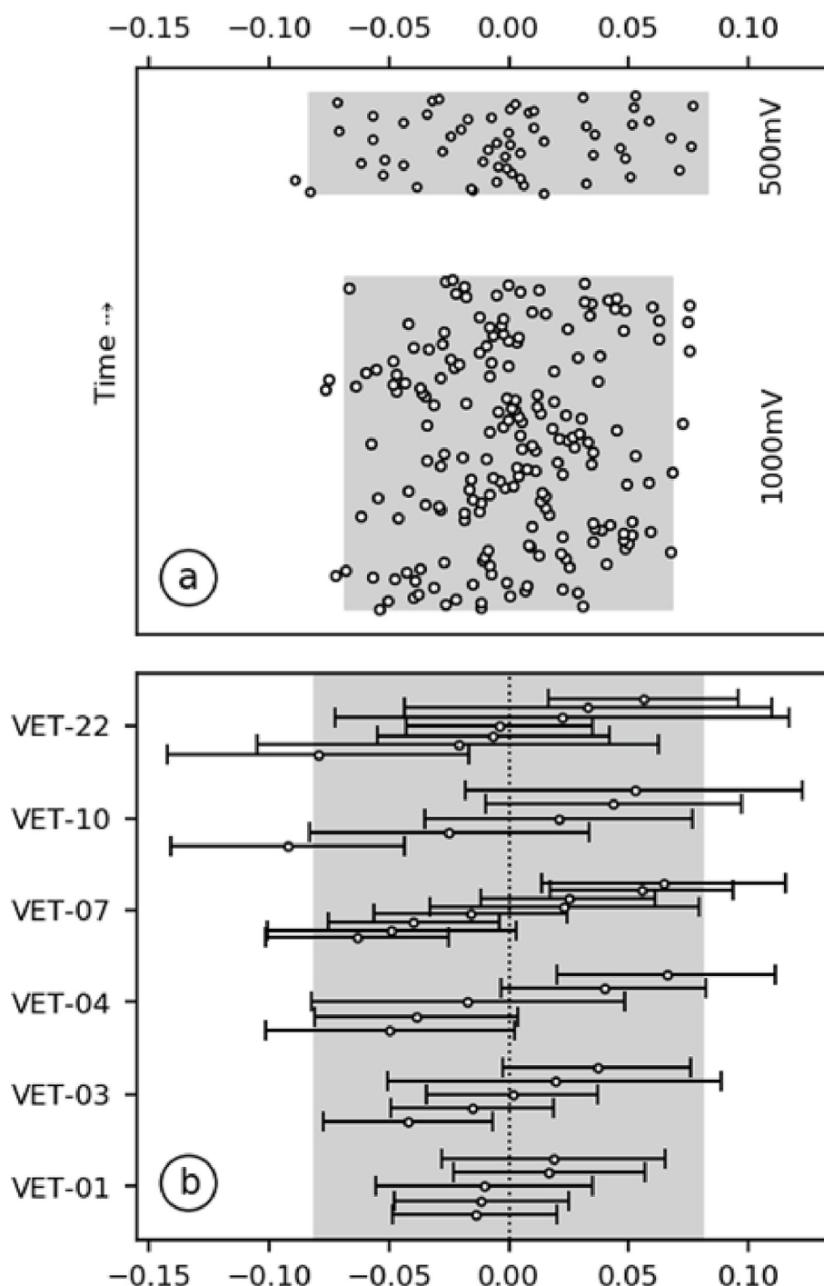
Fig. 4. Reproducibility of \delta^{53}\text{Cr}_{\text{SRM979}} values of: (a) <individual analyses of SRM979 with 52Cr beam intensities of 500 mV and 1000 mV, respectively. Gray fields display 2\sigma intervals; (b) Repeated analyses of 5 samples processed separately through chemistry. Cr isotope compositions are shown as deviation from the respective sample means, errors are 2SE internal errors, and the gray field shows 2\sigma of the analyses of \pm 0.08\% .
