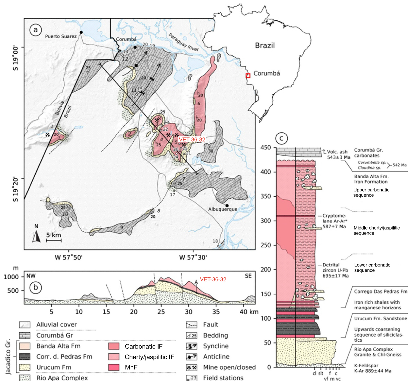
Fig. 1. Local geology of the Corumbá area: (a) Simplified geological map around Corumbá. Locations: 1, Morro do Jacadigo (Mutum); 2, M. da Tromba dos Macacos; 3, M. do Urucum; 4, M. Santa Cruz; 5, M. Grande; 6, M. do Rabichão; 7, M. do Zanetti; 8, M. Pelada; 9, M. d'Aguassu; 10, M. do Sajutá; 11, Laginia Quarry; 12, Corral Quarry (Modified after (Angerer et al., 2016)). Location of drill hole VET-36-32, from which samples have been analyzed herein, is indicated (b) Simplified NE-SW striking profile, marked with barred line on (a); location of drill hole VET-36-32 is indicated. (c) Summarized stratigraphic profile, showing known radiometric ages published by (Babinski et al., 2013; Freitas et al., 2017; Piacentini et al., 2013). Details see text. cl = clay, slt = silt, vf = very fine, f = fine, m = medium, c = coarse, vc = very coarse.
