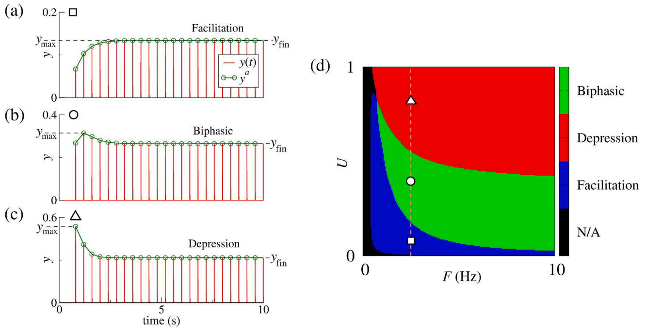
Fig. 2. (a–c) Dynamics of the active neurotransmitters in the synapse for three different regimes, (a) facilitation, (b) biphasic, and (c) depression. Red lines show the dynamics of active neurotransmitters represented by the y variable, and the green line with circles represents the y amplitude immediately after the spike event, y^a = y(0) . In Figs. (a–c), we consider F = 2.5 Hz, (a) U = 0.1 for facilitation, (b) U = 0.4 for biphasic, and (c) U = 0.8 for depression regime. In Figs. (a–c), the maximal value of y overtime is identified as y_{\max} while the final amplitude of y is represented by y_{\text{fin}} . (d) Regimes found in the dynamics synapses: facilitation, depression and biphasic. The facilitation and depression regimes are identified by means of Eqs. (45) and (46). If both conditions of Eqs. (45) and (46) are satisfied over time we identified the biphasic regime. The parameters U and F considered in Figs. (a–c) are indicated in Fig. (a). (For interpretation of the references to colour in this figure legend, the reader is referred to the web version of this article.)
