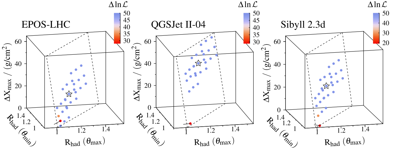
FIG. 9. Values of the modification parameters (points) for all possible combinations of experimental systematic uncertainties on the energy ( \pm 14\% ), X_{\text{max}} ( \pm 8 \text{ g/cm}^2 ), and S(1000) ( \pm 5\% ). The color of the points shows the difference in log-likelihood expressions ( \Delta \ln \mathcal{L} ) in the case of no modifications and in the case of the assumed template modifications, including the differences higher than 50 (note the slightly different scale between models). The results (see Table III) for no systematic shift of the data are highlighted by stars. Dashed lines outline the contour of the plane from the best-fit to the points. The closest approach to the nonmodified ( R_{\text{had}}(\theta) = 1 , \Delta X_{\text{max}} = 0 \text{ g/cm}^2 ) model predictions using a dense scan of linear combinations of experimental systematic uncertainties is connected with this point by a black line. The animated rotated views are available at [40].
