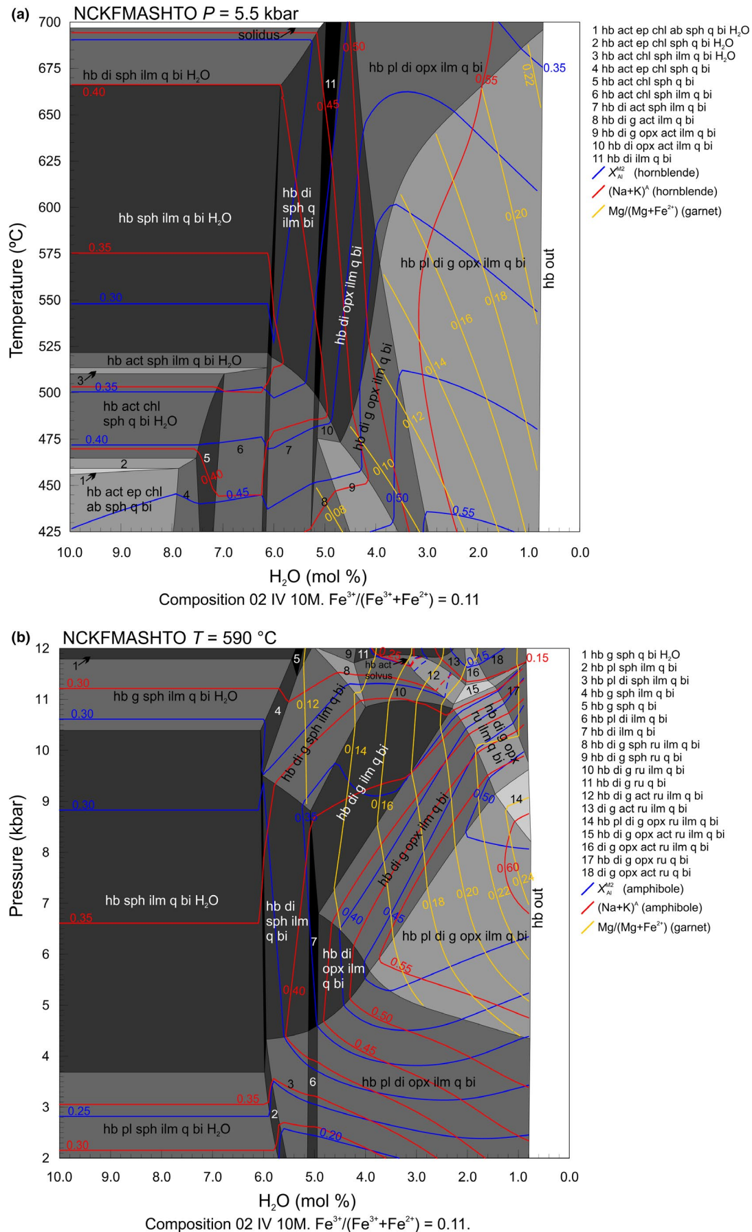
FIGURE 19 (a) T - X_{\text{H}_2\text{O}} pseudosection constructed for composition 02-IV-10M. (b) P - X_{\text{H}_2\text{O}} pseudosection constructed for composition 02-IV-10M
