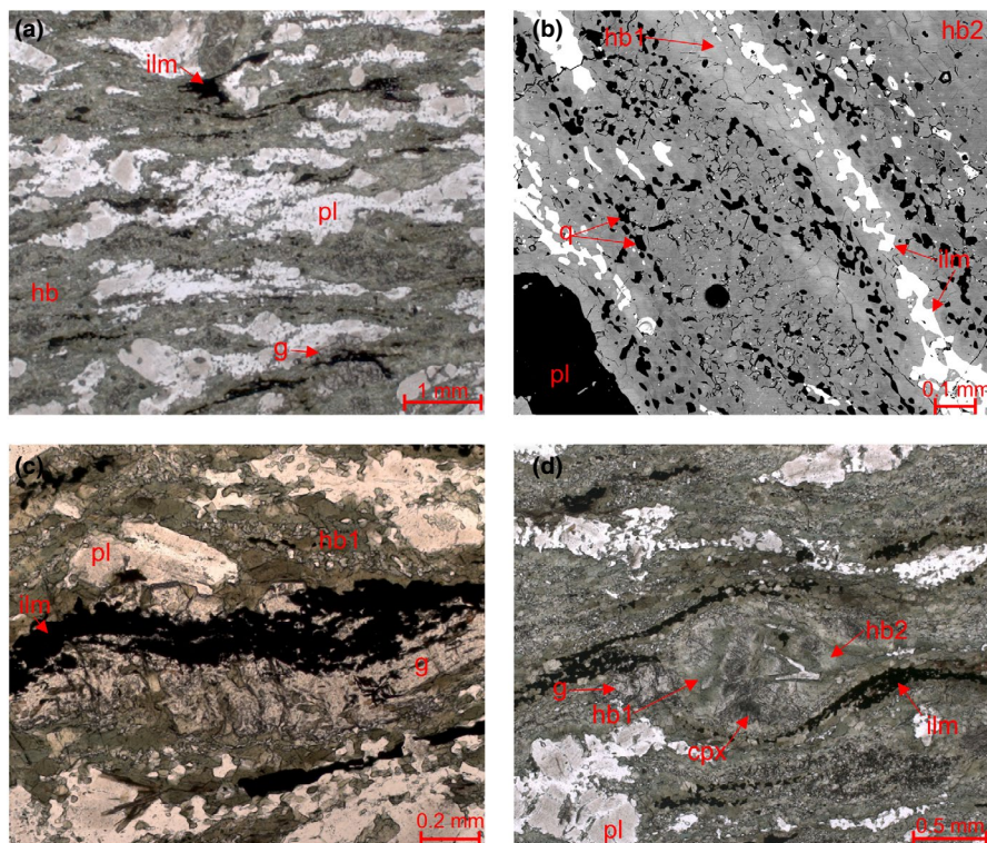
FIGURE 5 (a) General aspect of the lineated metagabbro. (b) Hornblende aggregate in lineated metagabbro. Backscattered electron image. (c) Elongate garnet crystal in lineated metagabbro. (d) Clinopyroxene crystal, partially replaced by actinolitic hornblende and wrapped around by the lineation
