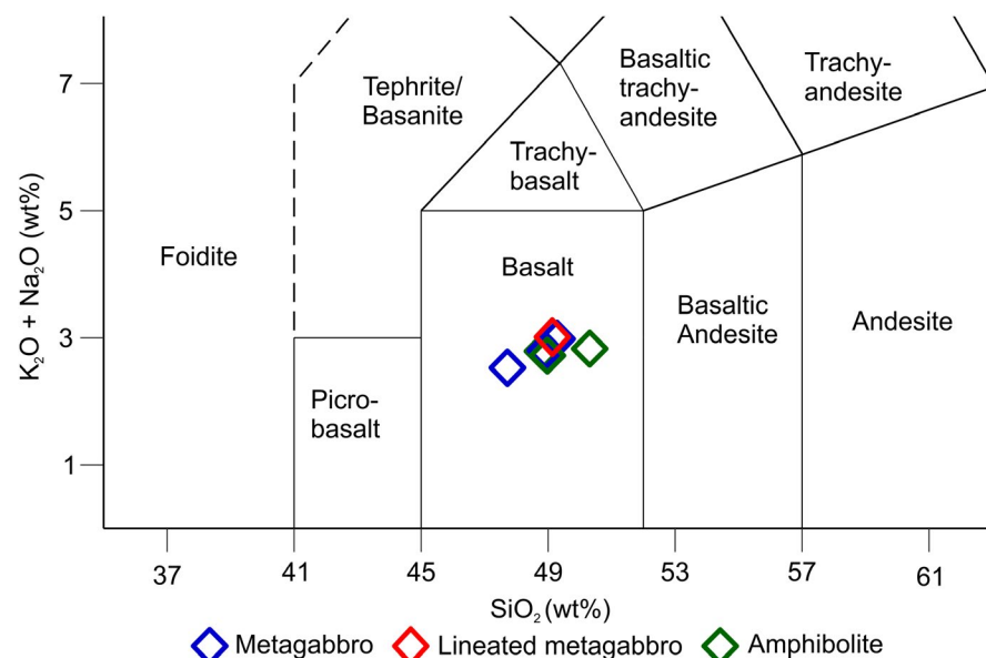
FIGURE 2 Chemical compositions of the studied samples plotted on the diagram for classification of volcanic rocks of Le Maitre et al. (1989)
