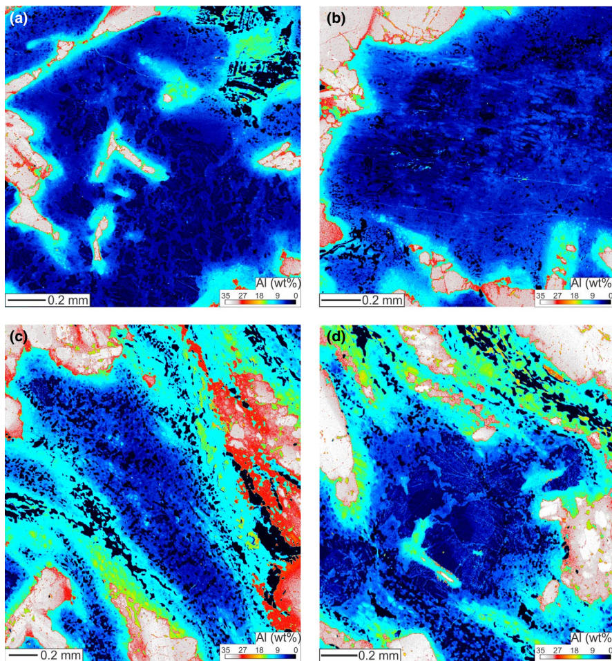
FIGURE 9 WDS compositional maps showing the abundance of Al in textures from metagabbro and lineated metagabbro samples. Black areas correspond to pyroxene, quartz or cummingtonite, white to red areas correspond to plagioclase, while dark blue to green areas correspond to hornblende. (a, b) metagabbro samples. (c, d) Lineated metagabbro samples
