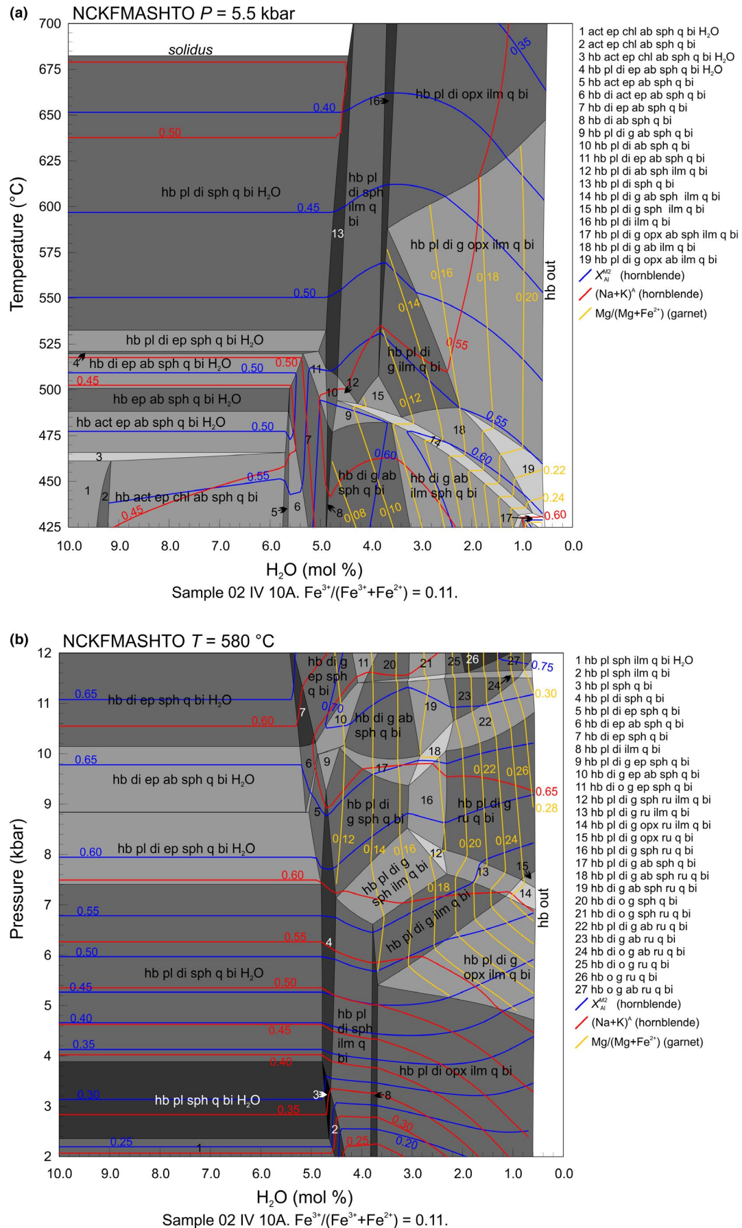
FIGURE 18 (a) T - X_{\text{H}_2\text{O}} pseudosection constructed for composition of sample 02-IV-10A. (b) P - X_{\text{H}_2\text{O}} pseudosection constructed for composition of sample 02-IV-10A
