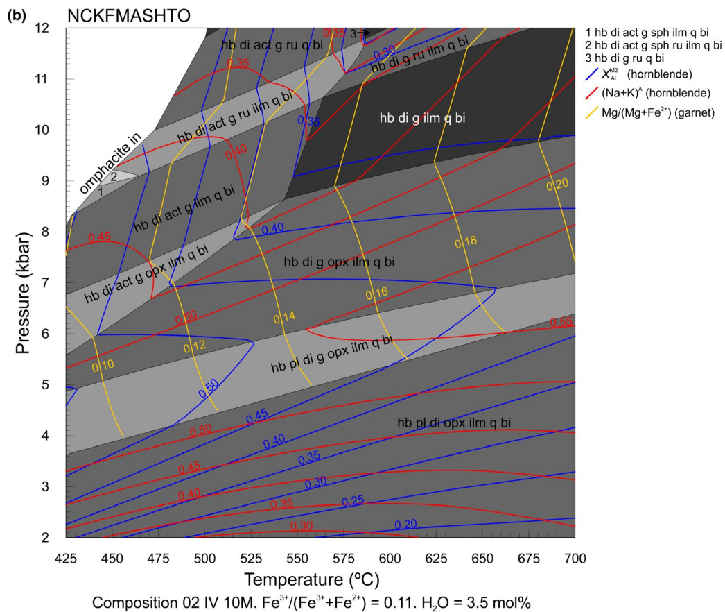
FIGURE 20 P - T pseudosections constructed for the composition of sample 02-IV-10A (a) and for composition 02 IV 10M (b), assuming \text{H}_2\text{O} = 3.5 \text{ mol}\%
