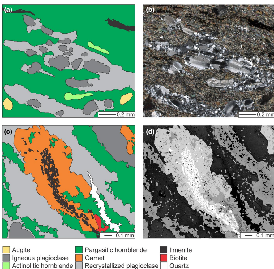
FIGURE 6 Textural features in lineated metagabbro samples, as simplified sketches (left) and photomicrographs or backscattered electron images (right). (a, b) Igneous plagioclase remnants in metamorphic plagioclase aggregate in lineated metagabbro sample. (c, d) Ilmenite mantled by garnet in lineated metagabbro sample
