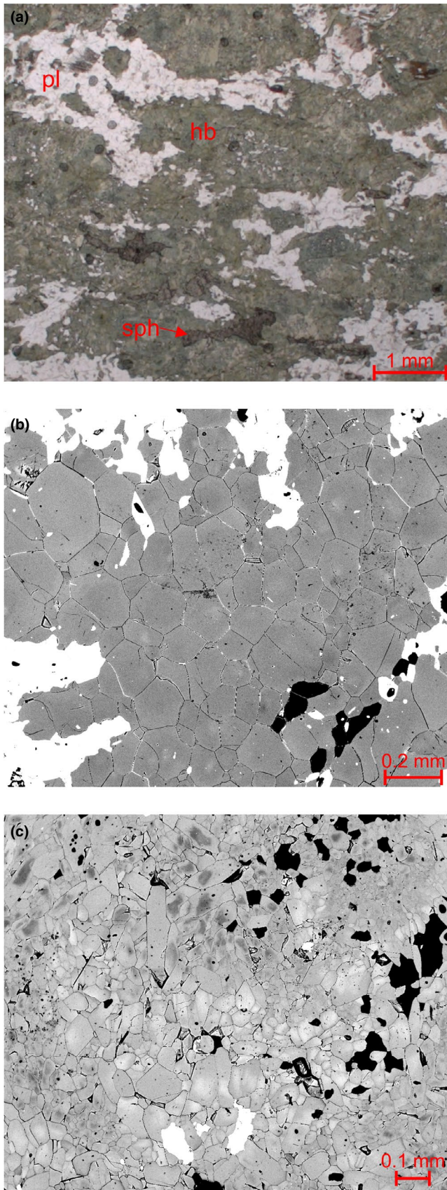
FIGURE 7 (a) General aspect of the amphibolite. (b) Polygonal plagioclase crystals in amphibolite sample. (c) Polygonal pargasitic hornblende crystals in amphibolite sample. Note the presence of two types of zoning: with actinolitic (darker) cores (top-centre, up left corner) and with pargasitic (brighter) cores (bottom-centre). Both b and c are backscattered electron images
