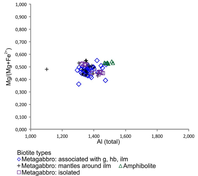
FIGURE 14 Chemical variation of biotite
