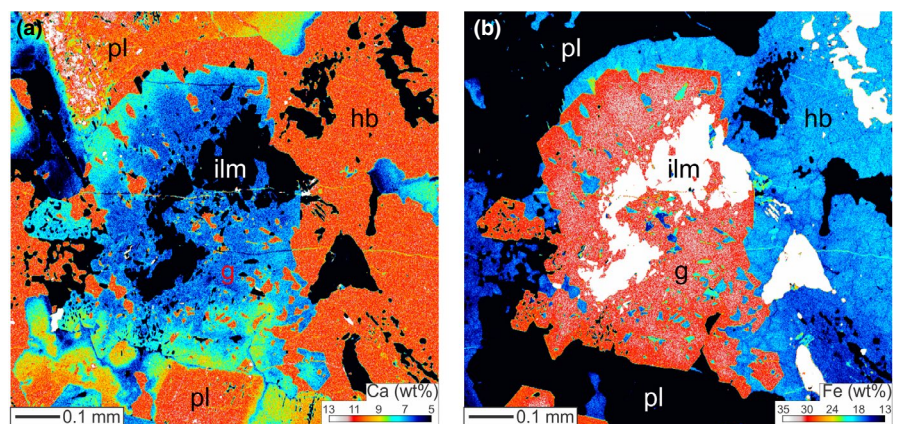
FIGURE 13 WDS compositional maps of a garnet crystal from a metagabbro sample, showing abundances of calcium (a) and iron (b)
