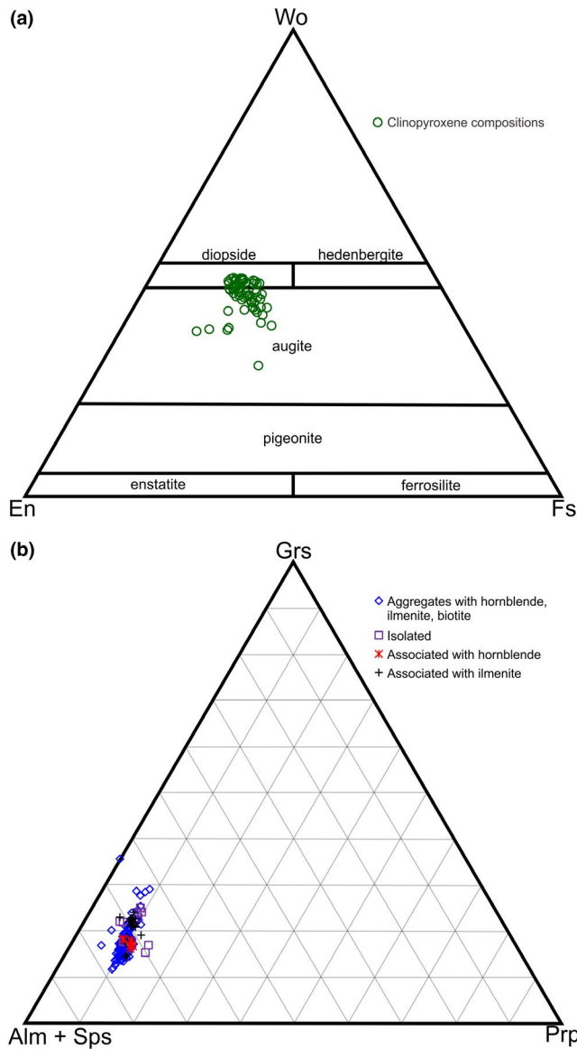
FIGURE 12 Chemical variation of clinopyroxene and garnet
