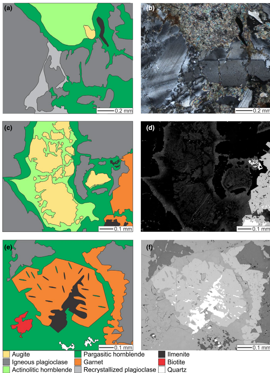
FIGURE 4 Textural features in metagabbro samples, as simplified sketches (left) and photomicrographs or backscattered electron images (right). (a, b) Actinolitic hornblende pseudomorph after clinopyroxene, mantled by pargasitic hornblende (top), metamorphic plagioclase at igneous plagioclase rims (centre-left) and ilmenite crystal mantled by pargasitic hornblende (top-right). (c, d) clinopyroxene crystal partially replaced by actinolitic hornblende and mantled by pargasitic hornblende. (e, f) Ilmenite mantled by garnet, and garnet in contact between hornblende and plagioclase
