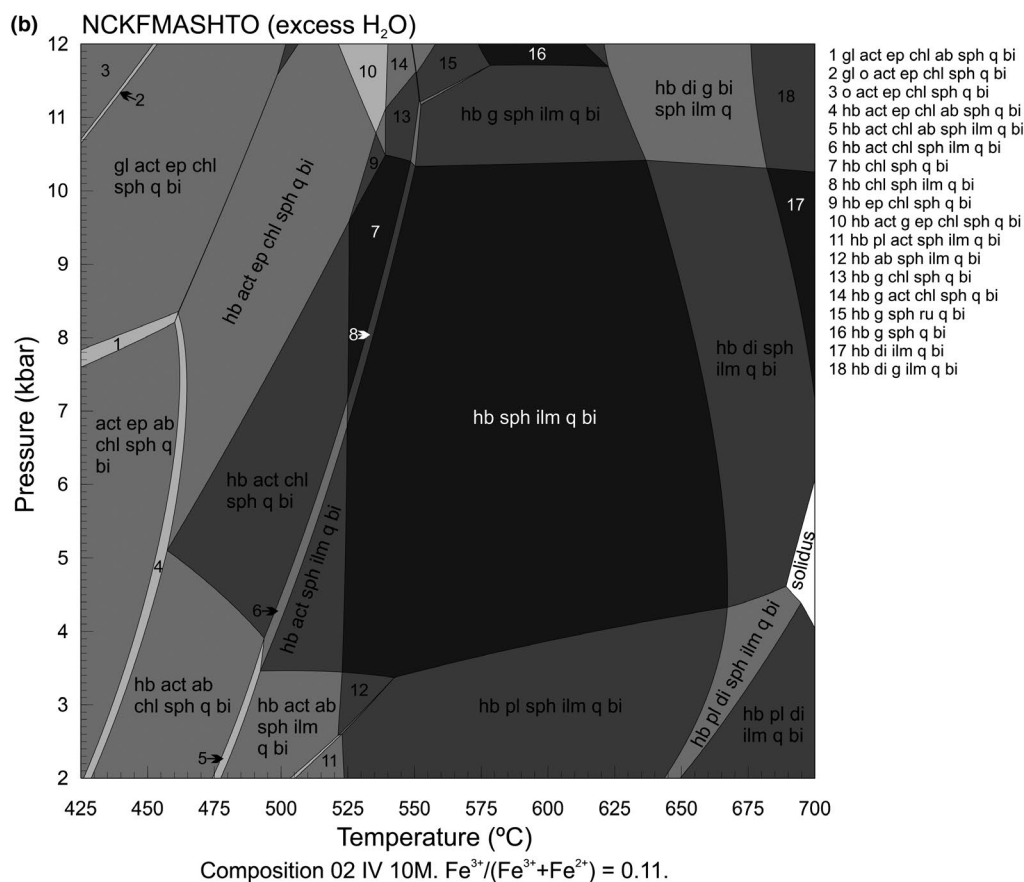
FIGURE 17 P - T pseudosections constructed for the composition of sample 02-IV-10A (a) and for composition 02 IV 10M (b)
