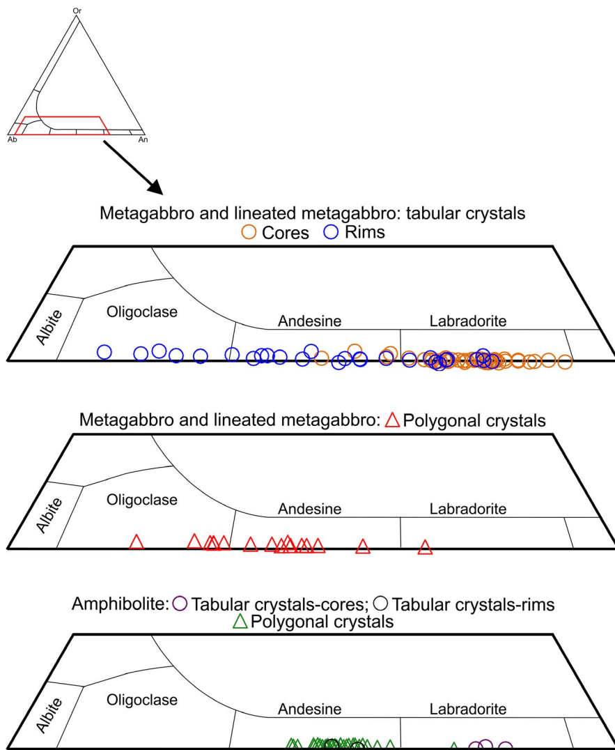
FIGURE 11 Chemical variation of plagioclase
