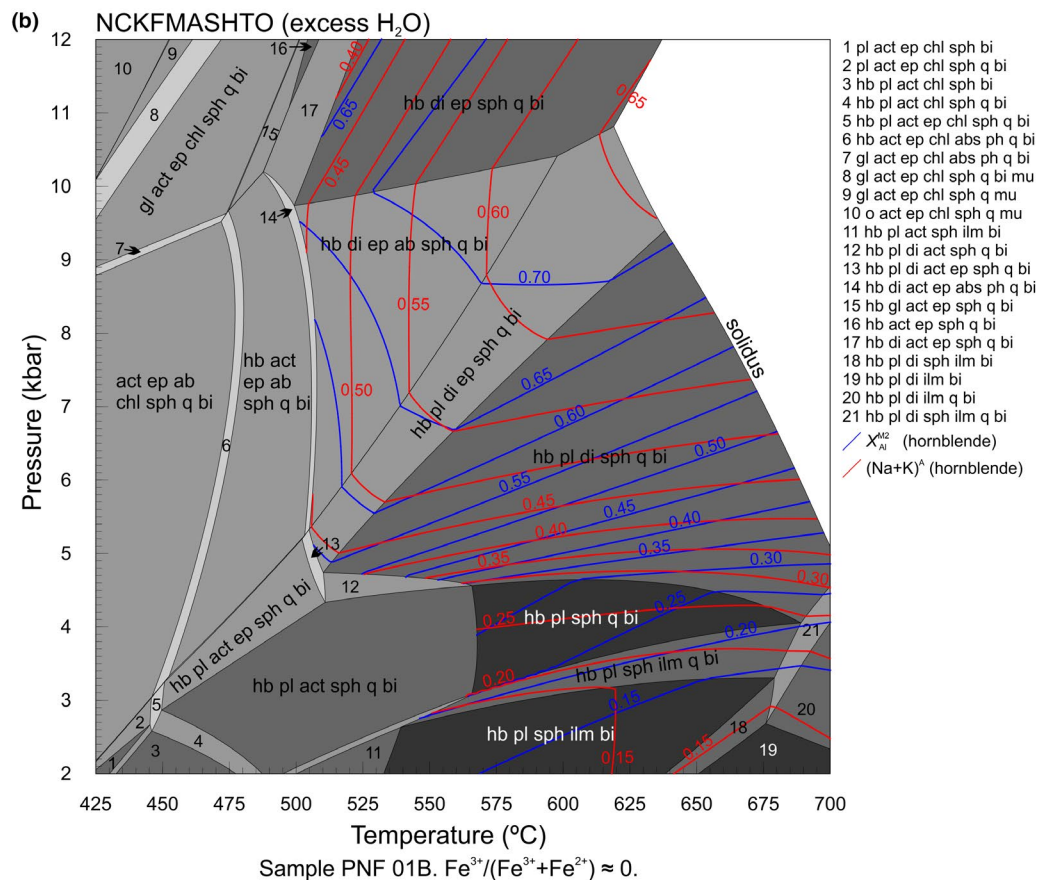
FIGURE 16 P - T pseudosections constructed for the composition of sample PNF 01B, assuming X_{Fe^{3+}} = 0.09 (a) and X_{Fe^{3+}} \approx 0 (b)
