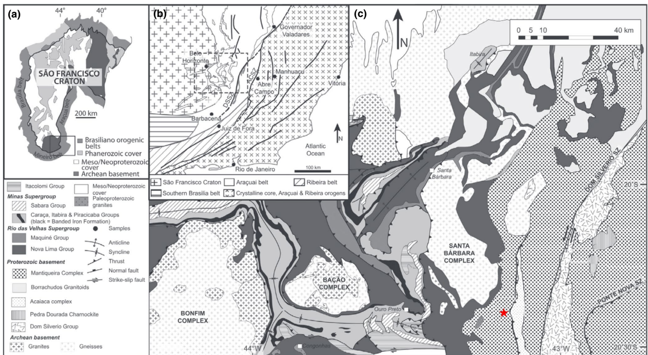
FIGURE 1 Geological context of the studied samples. The red star marks the location of the studied samples. Maps by Cutts et al. (2018)
