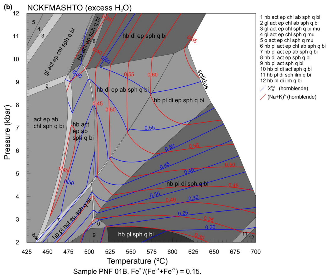
FIGURE 15 P - T pseudosections constructed for the composition of sample PNF 01B, assuming X_{\text{Fe}^{3+}} = 0.18 (a) and X_{\text{Fe}^{3+}} = 0.15 (b)
