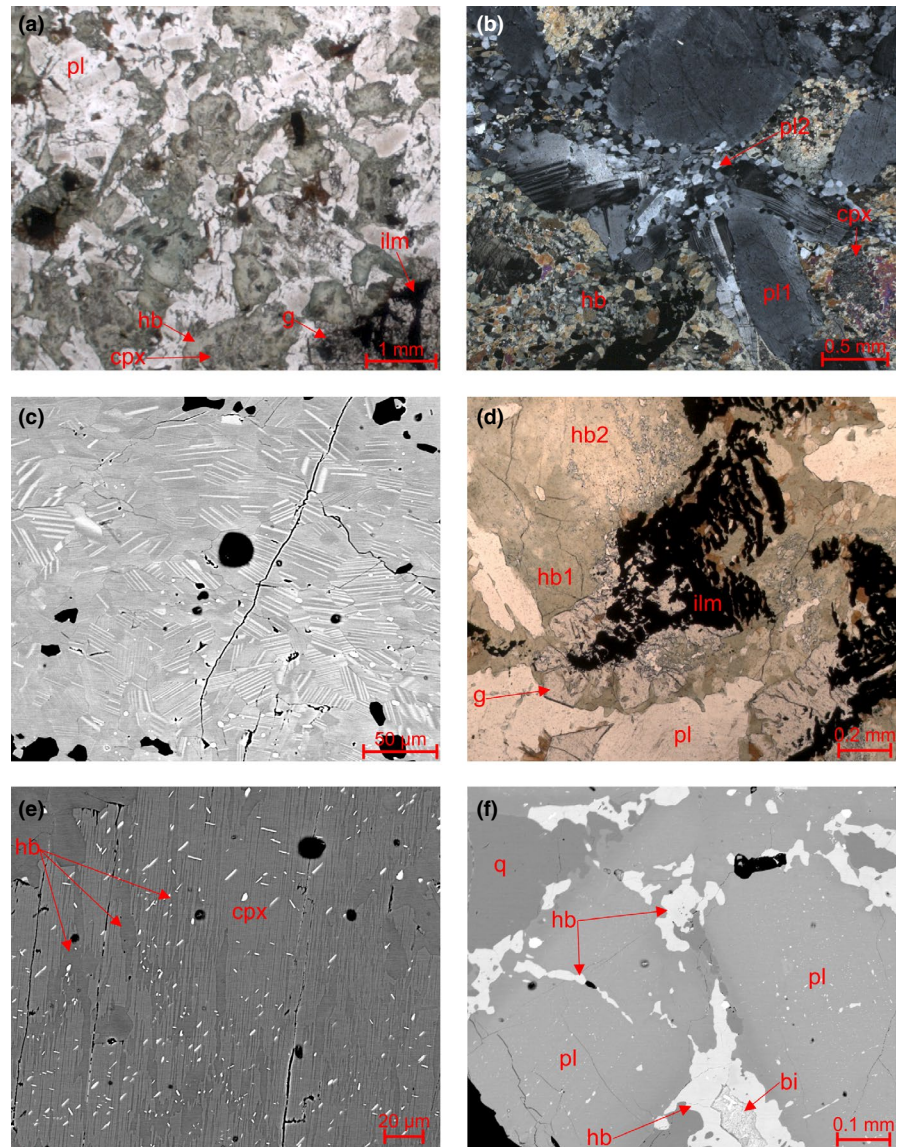
FIGURE 3 (a) General aspect of the metagabbro. (b) Fine-grained plagioclase in the rims of tabular, igneous plagioclase. (c) Cumingtonite exsolution lamellae (brighter) in actinolitic hornblende crystals (darker) in metagabbro sample. Backscattered electron image. (d) A combination of different reaction textures in a metagabbro sample: part of the ilmenite aggregate is mantled by garnet (bottom) and part is mantled by pargasitic hornblende (top). The pargasitic hornblende mantle actually separates the ilmenite aggregate from an actinolitic hornblende pseudomorph after clinopyroxene (top-left). (e) Replacement of pyroxene by actinolitic hornblende along micrometric planes in metagabbro sample. Backscattered electron image. (f) Pargasitic hornblende in fractures and contacts between plagioclase crystals in metagabbro sample. Backscattered electron image
