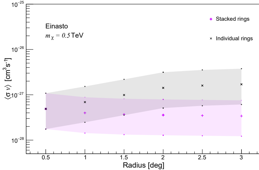
Figure 16. Median 95% C.L. exclusion limits (black ‘ \times ’) and their 1\sigma variance (grey shading) on the DM annihilation cross section that result from RoIs consisting of individual rings centered on the GC, with width 0.5^\circ and outer edge at the stated radius. Purple ‘+’ symbols and shadings indicate the corresponding limits when instead combining all rings up to the stated radius. All limits are based on a DM mass of m_\chi = 0.5 TeV DM and an Einasto profile for the DM distribution.
