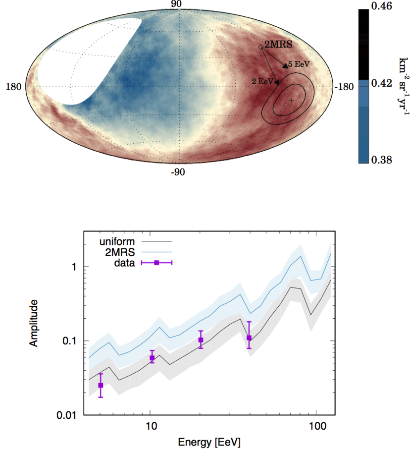
Figure 1: Top: measured cosmic-ray flux for events detected with energy above 8 EeV averaged on top-hat windows of 45^\circ , in Galactic coordinates [2]. The direction of the reconstructed dipole is shown together with the 68% and 95% C.L. regions. The 2MRS dipole direction is also shown as well as cosmic-ray expectations from 2MRS sources, taking into account magnetic deflections. Bottom: evolution of the dipole amplitude as a function of energy as well as expectations from two different extragalactic source scenarios [3].
