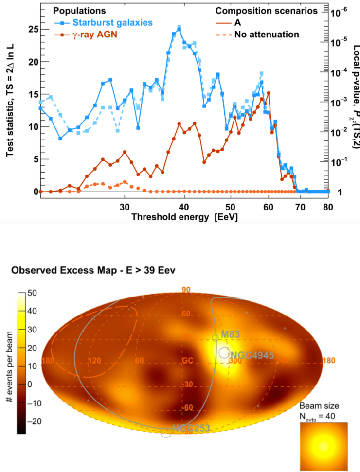
Figure 2: Top: test statistic (TS) as a function of the energy threshold for SBGs and \gamma -AGNs with and without take into account the attenuation of the intensity due to energy losses [5]. Bottom: observed excess map for starburst galaxies [5].
