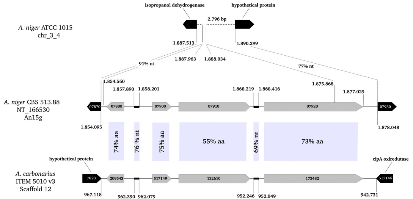
Fig. 1. Comparative sequence analysis of the putative ochratoxin gene cluster harboring PKS An15g07920 of A. niger strain CBS 513.88, and equivalent genomic regions of A. niger strain ATCC 1015 and A. carbonarius ITEM 5010 v3. Each line represents the genomic context of equivalent regions. Gray arrows represent genes within the cluster; and black arrows, bordering genes common to all genomes. Annotations ID either from JGI or NCBI are shown inside arrows. Genomic coordinates are depicted along the dotted lines. Amino acid sequence similarities between orthologs are shown within shaded areas as well as similarities in nucleotide sequences of intergenic regions. As indicated, A. niger strain ATCC 1015, carries a truncated version of An15g07920.
