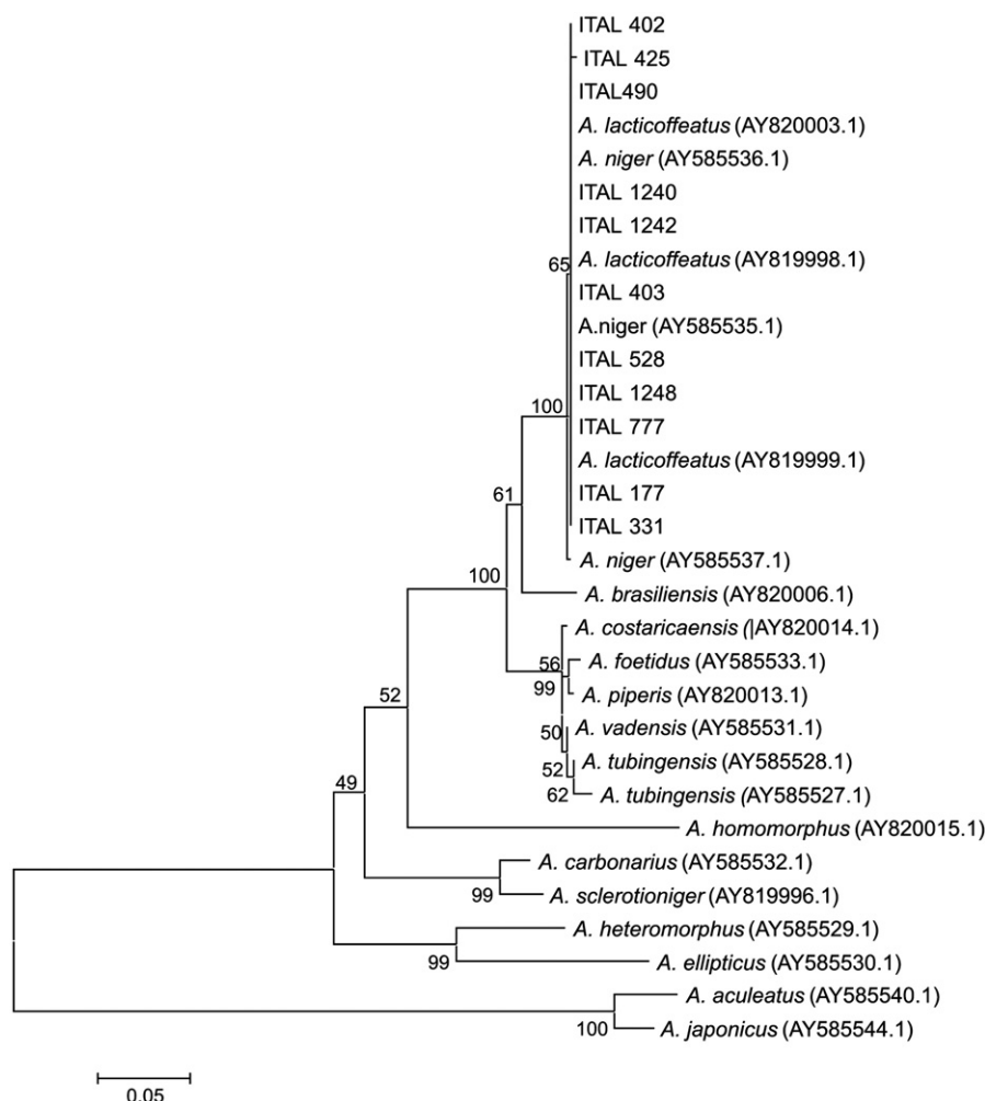
Fig. 3. A phylogenetic tree of Aspergillus from section Nigri based on \beta -tubulin gene sequences. Numbers above the branches correspond to bootstrap values generated by CLUSTAL X 1.6.
