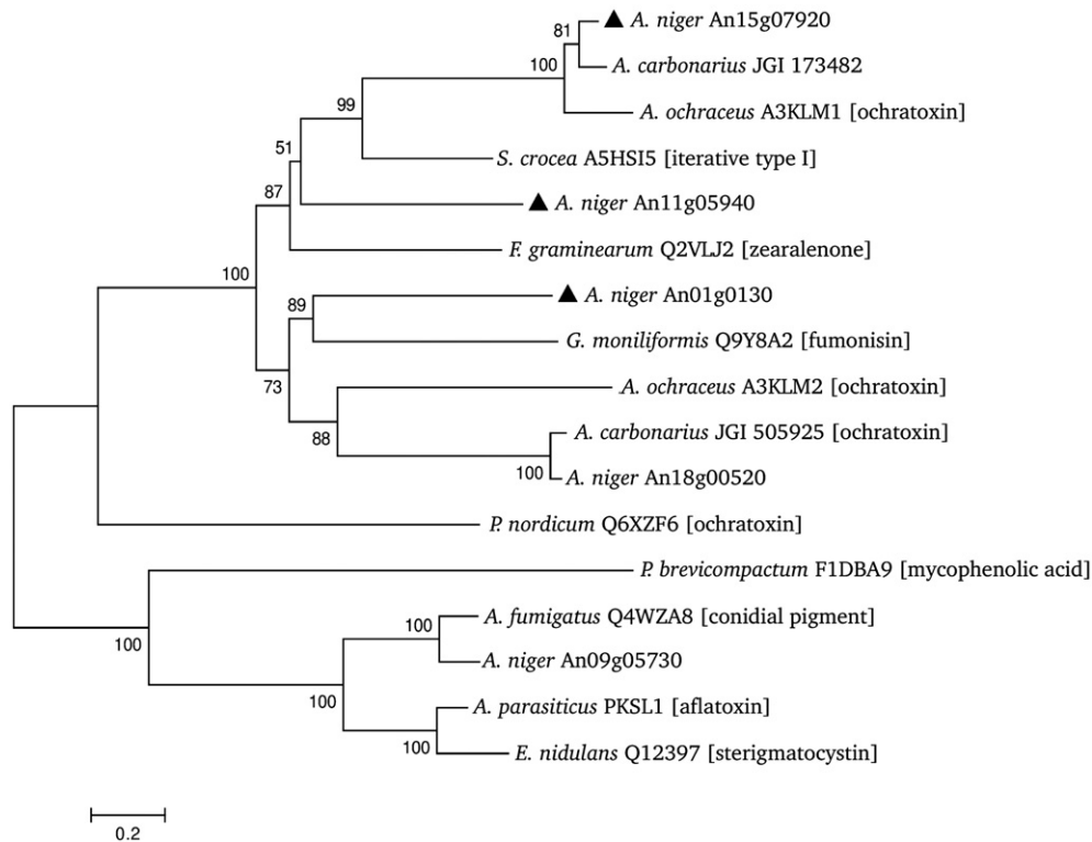
Fig. 2. Sequence similarity relationships among selected PKSs. Type I PKSs were selected from different organisms and various predicted functions in addition to five PKSs of A. niger and two of A. carbonarius . Black triangles represent pks genes missing in A. niger strain ATCC 1015. The tree was inferred by Neighbor-joining analysis, with distances computed using the JTT matrix-based method and bootstrap consensus tree from 1000 replicates. Analyses were conducted in MEGA5 (Tamura et al., 2011).
