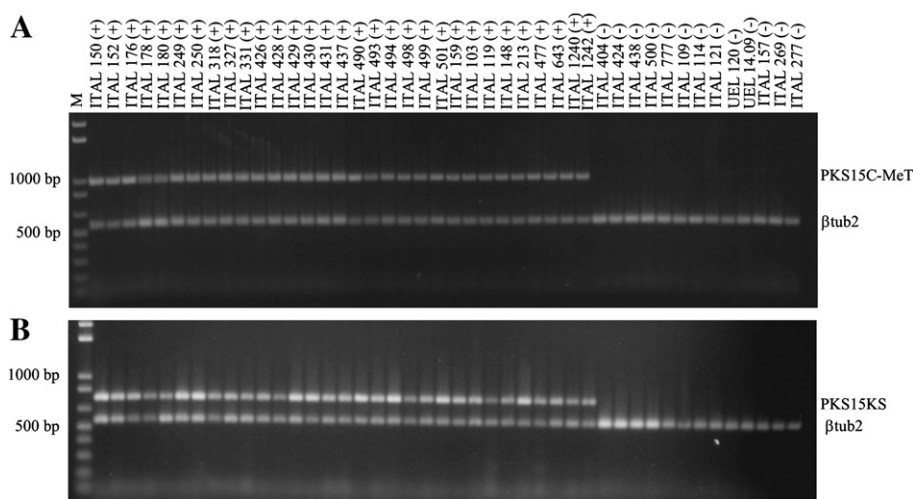
Fig. 4. Association between An15g07920 and OTA production capability of each strain, as demonstrated by PCR performed with two primer pairs, PKS15C-MeT (A) and PKS15KS (B). PCR detected a 998 bp band and a 776 bp band, respectively, in the ochratoxin producing strains only. The 554 bp-amplicon corresponding to the βt2 region of the β-tubulin gene confirm the presence of PCR-compatible DNA in all strains.
