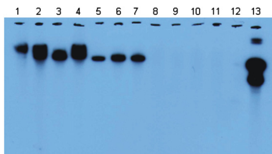
Fig. 5. Association between An15g07920 and OTA production capability of each strain, as demonstrated by Southern blot analysis of randomly selected A. niger OTA producing (lanes 1–7) and OTA non-producing strains (lanes 8–12). For hybridization, a fragment of the pks gene was labeled with ^{32} P and used for the assay. Lane 13 shows the plasmid with the probe, which served as the positive control.
