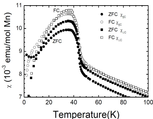
FIGURE 3. \chi vs. T of the zero-field-cooled (solid) and field-cooled (open) taken in 3.5 kOe for \text{BiMn}_2\text{O}_5 . Solid circles \chi_{\parallel} ; squares \chi_{\perp} .
