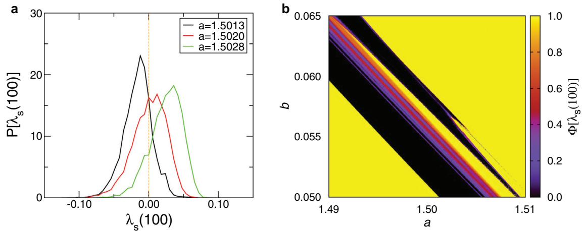
Fig. 4. (a) Histogram of the largest transversal finite time Lyapunov exponents ( \lambda_s(100) ) for a = 1.5013 (black line), a = 1.5020 (red line), and a = 1.5028 (green line). (b) Parameter space where the colour bar represents the fraction of positive values of \Phi(\lambda_s) . (For interpretation of the references to colour in this figure legend, the reader is referred to the web version of this article.)
