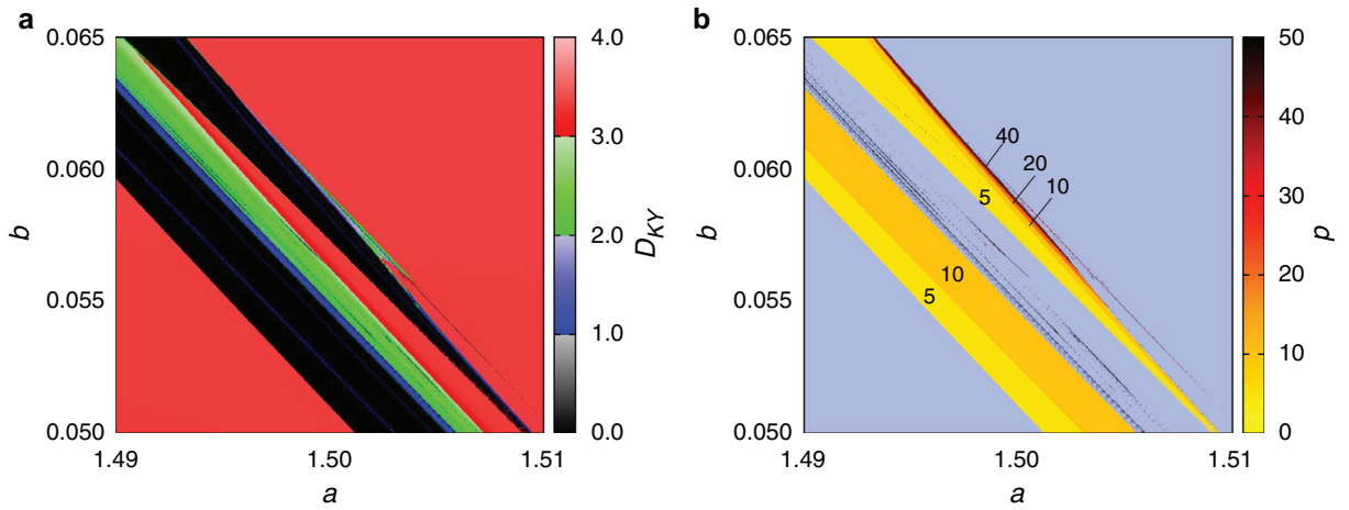
Fig. 3. Magnification of the parameter space marked by the yellow rectangle in Fig. 2(b), where the colour code in (a) represents the Kaplan-Yorke dimension, and in (b) represents the period of stable periodic orbits. (For interpretation of the references to colour in this figure, the reader is referred to the web version of this article.)
