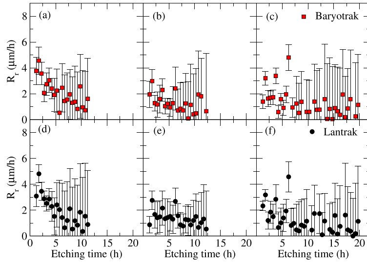
Fig. 2. Radial etch rates as function of the etching time for Baryotrak (red squares) and Lantrak (black dots) CR-39 detectors obtained at 80 °C for KOH ((a) and (d)), NaOH ((b) and (e)), and NaOH + ethyl alcohol ((c) and (f)) etching solutions.
