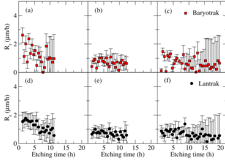
Fig. 3. Radial etch rates ( R_r ) as function of the etching time for Baryotrak (red squares) and Lantrak (black dots) CR-39 detectors obtained at 70 °C for KOH ((a) and (d)), NaOH ((b) and (e)), and NaOH + ethyl alcohol ((c) and (f)) etching solutions.
