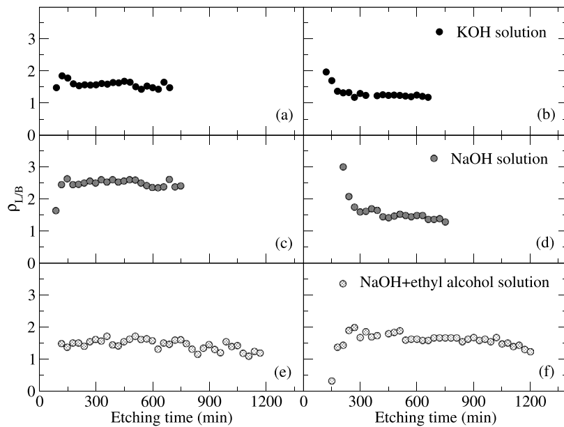
Fig. 5. Alpha track density ratio ( \rho_{L/B} ) as function of the etching time for the three aqueous solution at (a), (c), (e) 80 °C and (b), (d), (f) 70 °C.
