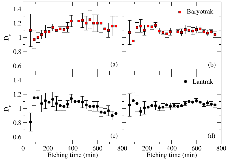
Fig. 1. Ratios of etch pit diameters ( D_r ) in detectors etched with NaOH + ethyl alcohol aqueous solution and NaOH (a) Baryotrak 80 °C, (b) Baryotrak 70 °C, (c) Lantrak 80 °C, and (d) Lantrak 70 °C.
