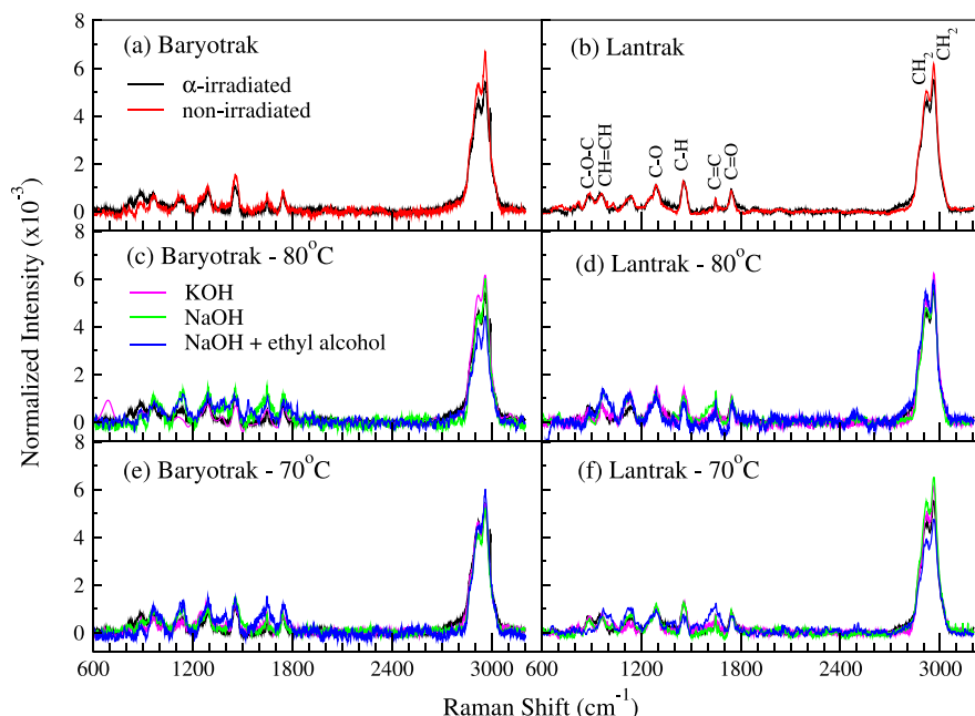
Fig. 7. Raman measurements for Lantrak and Baryotrak CR-39 detectors etched using KOH, NaOH and NaOH + ethyl alcohol at 80 °C and 70 °C compared with results obtained with non-irradiated and \alpha -irradiated detectors.
