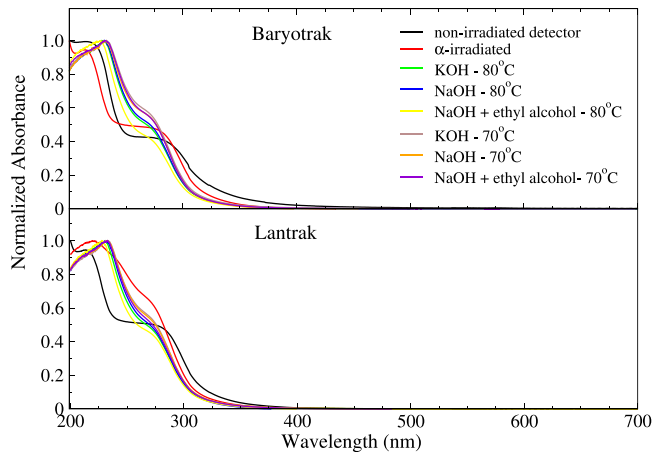
Fig. 6. Normalized absorbance spectra obtained from UV-Vis measurements for non-irradiated, \alpha -irradiated and \alpha -irradiated/etched detectors.
