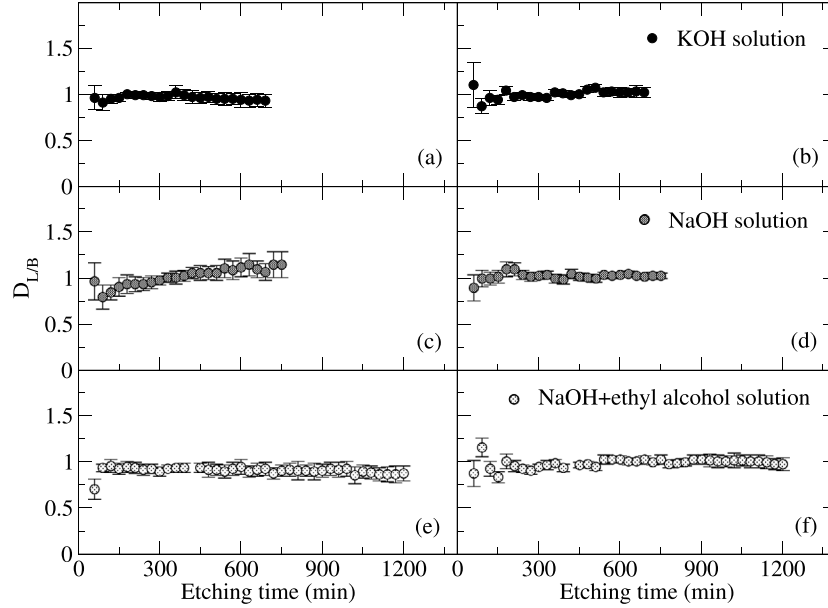
Fig. 4. Alpha track diameter ratio ( D_{L/B} ) as function of the etching time for the three aqueous solutions at (a), (c), (e) 80 °C and (b), (d), (f) 70 °C.
