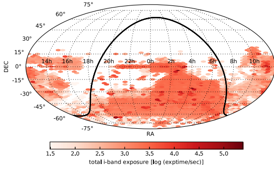
Fig. 1. Existing i -band coverage of the sky from DECam imaging as of March 2019.
