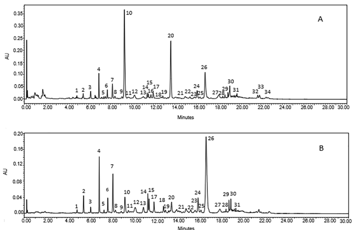
Fig. 1. Chromatogram representative of the sample mix of lemon, lime and rangpur citrus fruits. (A) Chromatogram recovered at 260 nm. (B) Chromatogram recovered at 350 nm.
