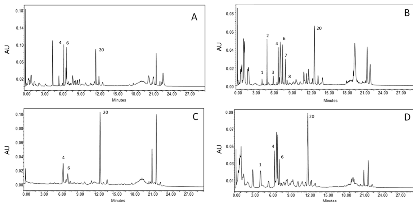
Fig. 3. Chromatograms obtained at 350 nm from (A) orange, (B) sweet orange, (C) tangerine ponkan and (D) tangerine.
