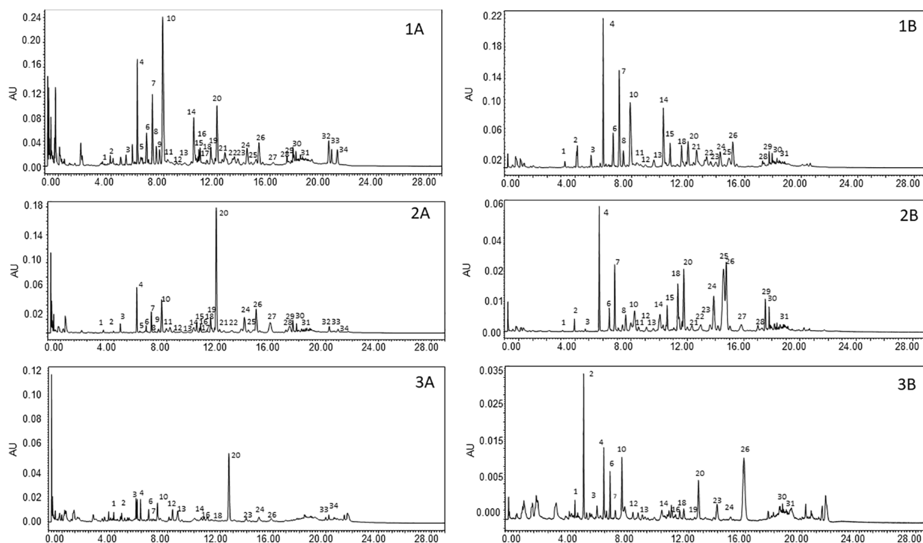
Fig. 2. Chromatograms obtained at 260 nm (A) and 350 nm (B) from (1) lemon, (2) lime and (3) rangpur lime.
