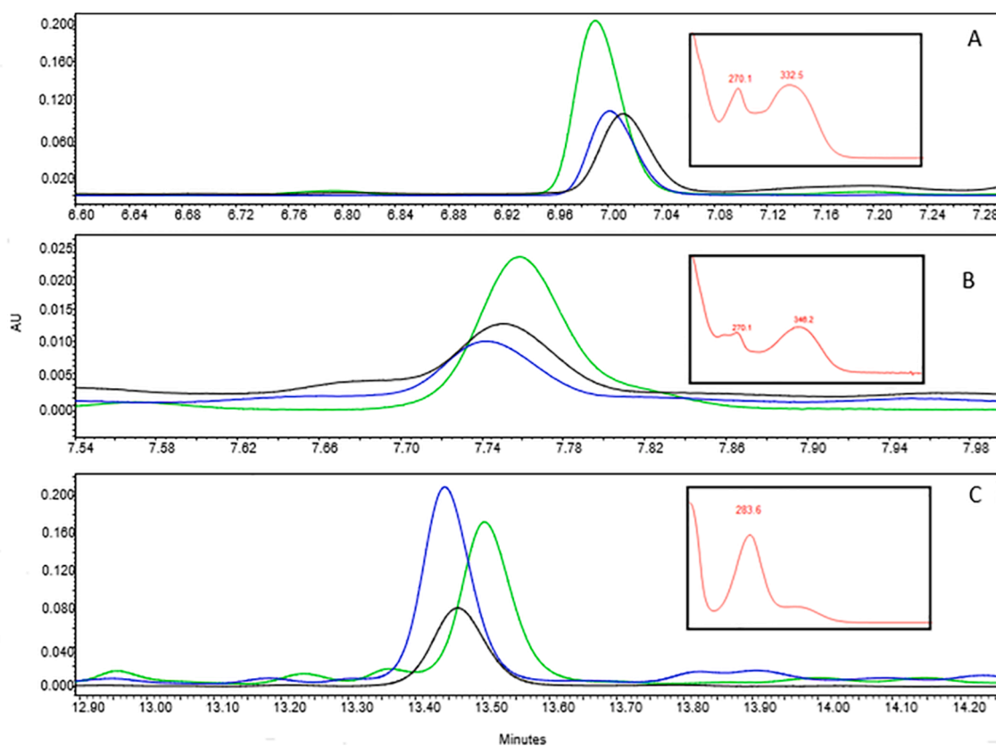
Fig. 4. Effect of sample matrix on the retention time in chromatograms recovered at 350 nm. (A) represents vicenin-2, (B) stellarin and (C) hesperidin. Green, black, and blue lines represent the peels samples of lemon, lime, and rangpur lime, respectively. (For interpretation of the references to colour in this figure legend, the reader is referred to the web version of this article.)
