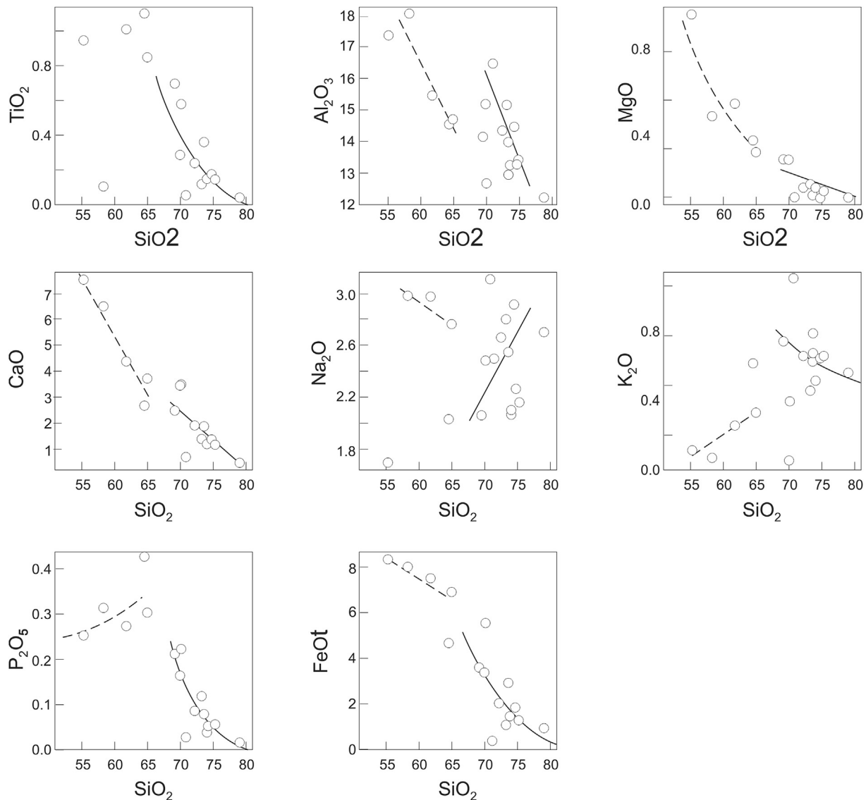
Fig. 3. Harker diagrams of major elements.
