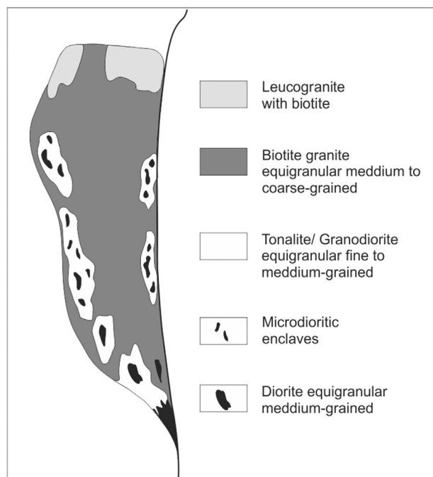
Fig. 14. Textural variation of the batholith, highlighting the lips in the basal portion rich in microdioritic enclaves and mafic minerals with finer texture than the dominant granite.
