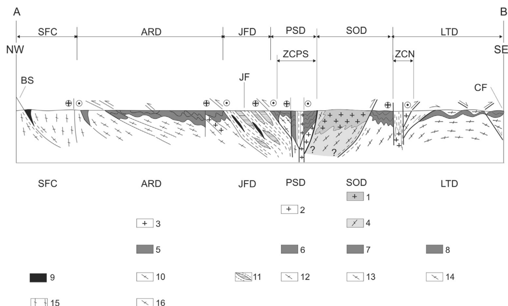
Fig. 12. NW-SE geological section of the Central Ribeira belt showing the positive-flower structure and tectonic contacts between the main terranes of the belt (adapted from Machado and Endo, 1993). Legend: 1 = Serra dos Órgãos batholith; 2 = Serra das Araras; 3 = Serra do Lagarto pluton; 4 = Rio Negro arc; 5 = Andrelândia Group; 6 = Supracrustal Paraíba do Sul; 7 = Santo Eduardo/Itaocara/Italva Formation/Group; 8 = Búzios Sequence; 9 = Bom Sucesso mafic-ultramafic sequence; 10 = Piedade Complex; 11 = Juiz de Fora; 12 = Quirino Complex; 13 and 14 = Rio dos Lagos Complex; 15 and 16 = Mantiqueira and Barbacena complexes.
