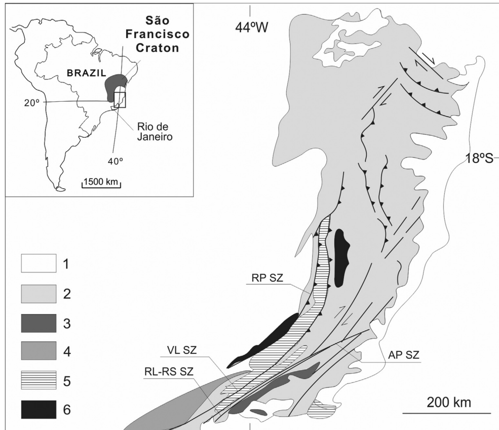
Fig. 1. Simplified map tectonic of the Ribeira belt. Adapted from Bizzi et al. (2003). 1 = Quaternary sediments; 2 = Brasiliano Orogenic System III; 3 = Serra dos Órgãos Batholith; 4 = Embu Terrane; 5 = Juiz de Fora Complex; 6 = Mantiqueira and Pocrane complexes. SZ = Shear Zones: RP = Rio Preto, VL = Valença, AP = Além-Paraíba, RL-RS = Ribeirão das Lajes-Rio Santana.
