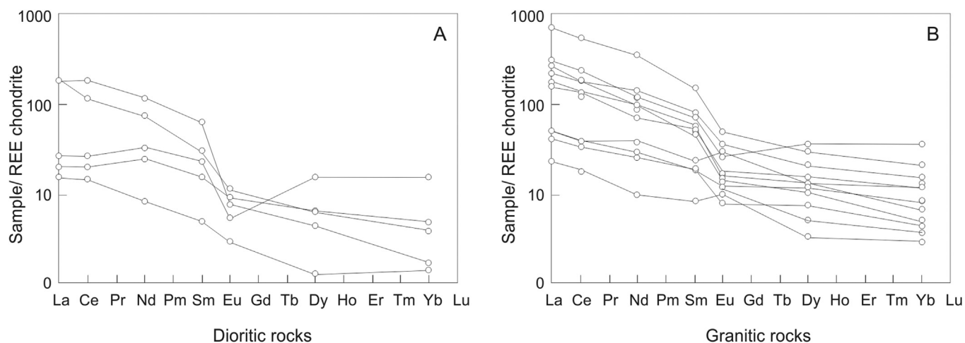
Fig. 8. Chondrite- normalized rare earth elements according to Sun and McDonough (1989).
