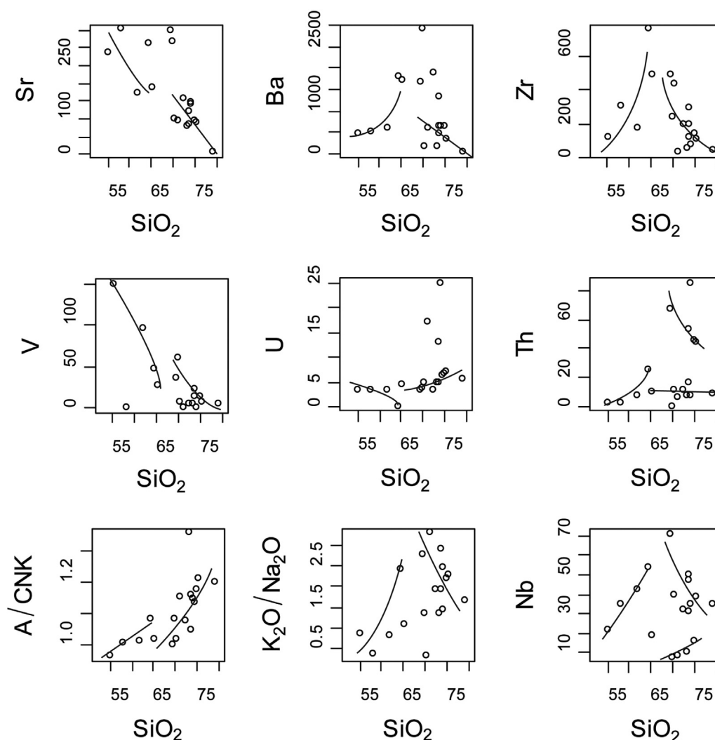
Fig. 4. Harker diagrams of trace elements.
