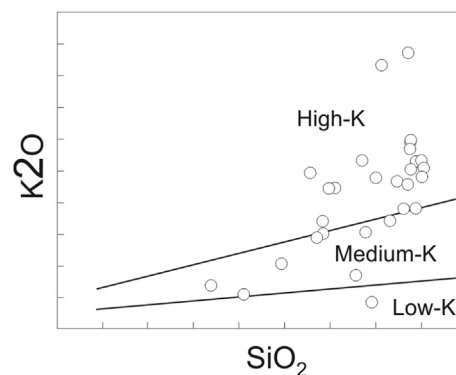
Fig. 7. K 2 O vs. SiO 2 , with fields after Le Maître (1989).
