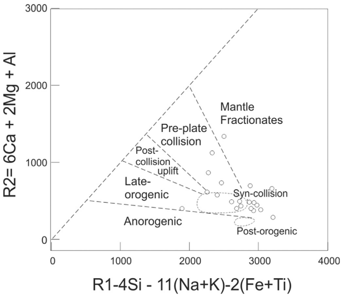
Fig. 11. R1-R2 diagram (Batchelor and Bowden, 1985).
