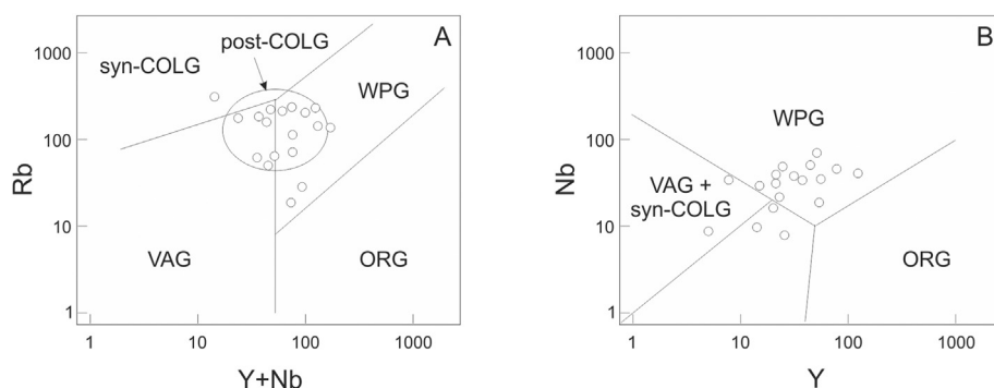
Fig. 10. Rb versus (Y + Nb) and Nb versus Y diagrams (Pearce et al., 1984; Pearce, 1996).
