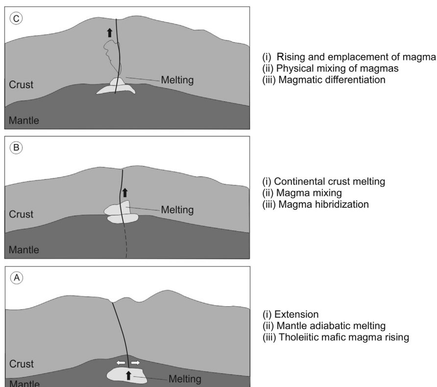
Fig. 13. Schematic model of the crust showing the generation of the Serra dos Órgãos Batholith: (a) Ductile shear zone reaching deep conditions and causing adiabatic melting of the mantle and generating a mafic magma; (b) Rise of mafic magma with increased of geothermal gradient in lower crust and partial melting of the rocks from the base of the continental crust; (c) Magma mixing with partial chemical interaction generating hybrid granitoids and areas rich in dioritic enclaves showing textural variation, highlighting the lips in the lower portion composed by areas rich in microdioritic enclaves associated with granitoids rich in mafic minerals and finer texture than the dominant granite.
