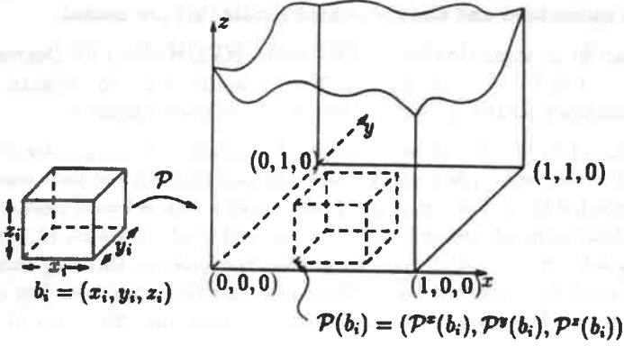
Figure 1: Packing of a box b_i = (x_i, y_i, z_i) into the box B = (1, 1, \infty) .
