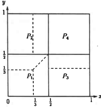
Figure 2: Subdivision of P_1, P_2 and P_3 .
