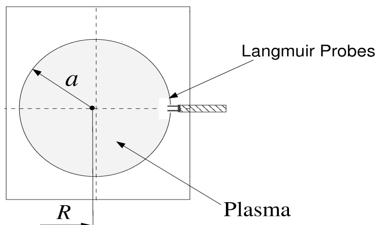
Figure 1. Cross section of the TCABR tokamak showing the Langmuir probes and plasma column.
