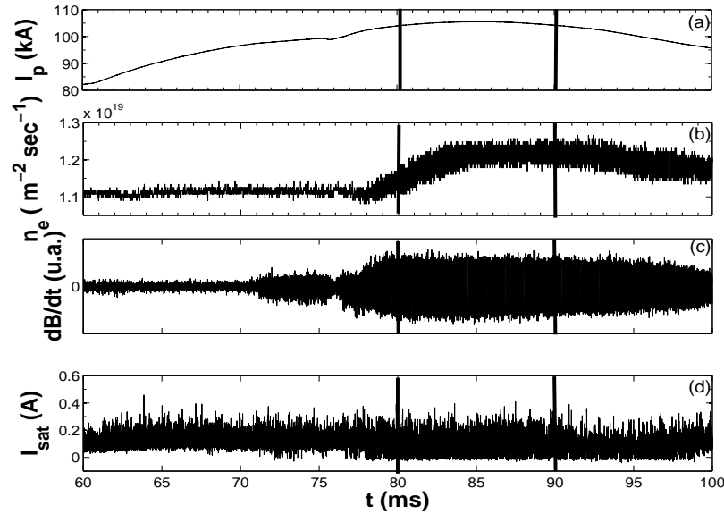
Figure 2. Time evolution of plasma discharge in TCABR tokamak. (a) Plasma current, (b) central chord plasma mean density, (c) magnetic oscillation, (d) ion current saturation. The vertical black lines indicate the analyzed time interval with high MHD activity.
