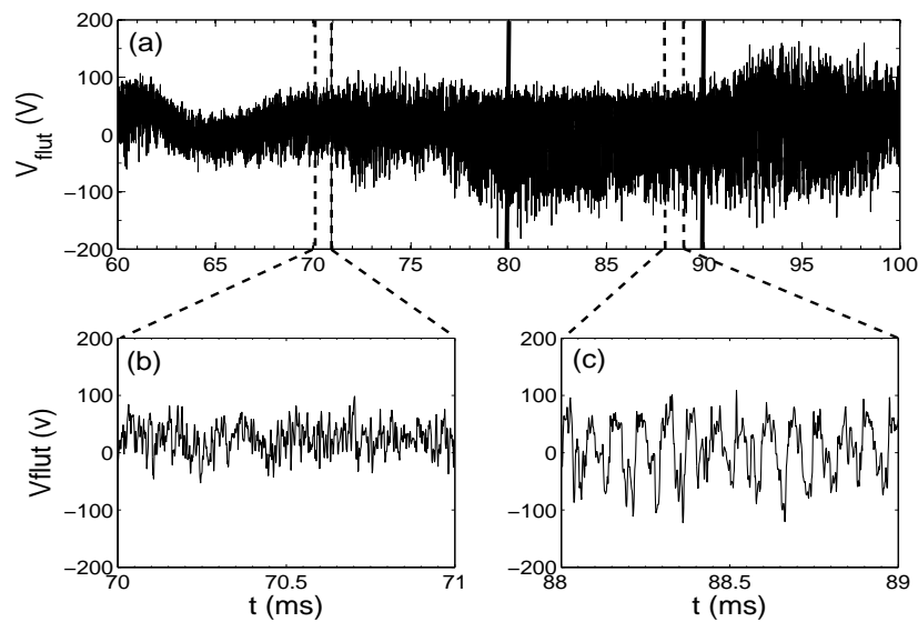
Figure 3. Time evolution of floating electrostatic potential fluctuation (a). Amplified time intervals with low MHD activity (b) and with high MHD activity (c) (dashed vertical lines). The vertical black lines indicate the analyzed time interval with high MHD activity.
