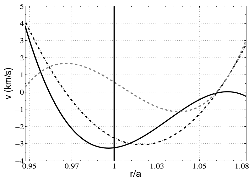
Figure 4. Radial profile of the averages phase (black line) and drift (dot-dashed line) velocities, and the difference between these velocities (dashed line)
