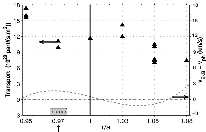
Figure 5. Radial profile of particle transport and the difference between the phase and flow velocities. Transport barrier localized on the shearless region on r/a = 0.97 (indicated by the vertical arrow).
