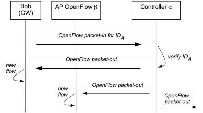
Fig. 5. OpenFlow messages for the new flow.
