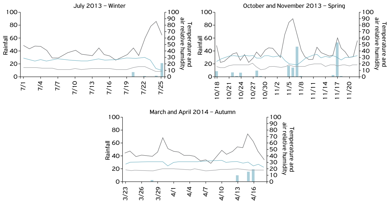
Figure 1. Daily data: rainfall (mm) (blue bar), maximum temperature (°C) (gray line), minimum temperature (°C) (purple line), air relative humidity (%) at 3 p.m. (blue line), during all seasons in Ribeirão Preto City, São Paulo state, Brazil.
