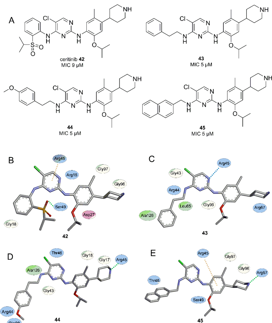
Figure 13. A) Chemical structure of ceritinib 42 and derivatives (43-45) synthesized as potential inhibitors of Mt DHFR. Main interactions of prepared compounds and Mt DHFR: B) ceritinib (38); C) 39; D) 40; E) 41. Interaction: orange dots: \pi -alkyl; blue dots: hydrogen bond; green dots: \pi -sigma (adapted from ref. 70). 3D images were drawn in Discovery Studio, Biovia.
