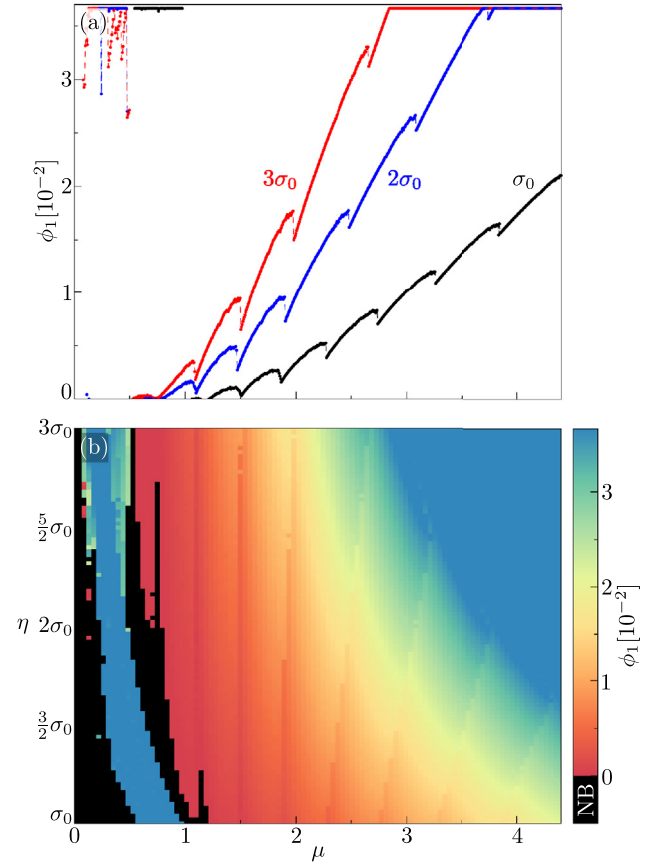
Fig. 7. Hill-like E_H(I) scenario: (a) approximated boundary of the \mu \times \phi_1 parameter space for \eta = \sigma_0 (black), 2\sigma_0 (blue) and 3\sigma_0 (red); (b) maximum value \phi_1 , up to the precision \delta\phi_1 = 5.0 \times 10^{-5} , at which the shearless edge transport barrier exists for the 100 \times 100 radial electric field configurations. In black colour, we indicate the cases in which no STB appears (Colour online).
