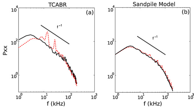
Fig. 8. Power spectrum of the floating potential fluctuation (a) and sandpile model (b) with (red) and without (black) high MHD activity. In the sandpile model we consider L = 200 , N_f = 3 , N_g = 3 , Z_c = 8 , \tau = 47 , 1.1 \times 10^6 iterations and 1.0 \times 10^6 transient iterations. In our simulations we consider N_{ext} = 0 to obtain black line and N_{ext} = 40 to red line. (For interpretation of the references to color in this figure, the reader is referred to the web version of this Letter.)
