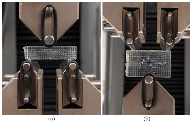
Fig. 14. The 3-point bending tests: cases (a) 3pb_1 and (b) 3pb_2.
