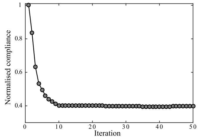
Fig. 5. Convergence plot for the cb_1 case.
