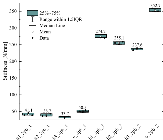
Fig. 15. Box plot of the experimental structural stiffness for cases 3pb_1 (with \bar{v} = 10\% ) and 3pb_2.
