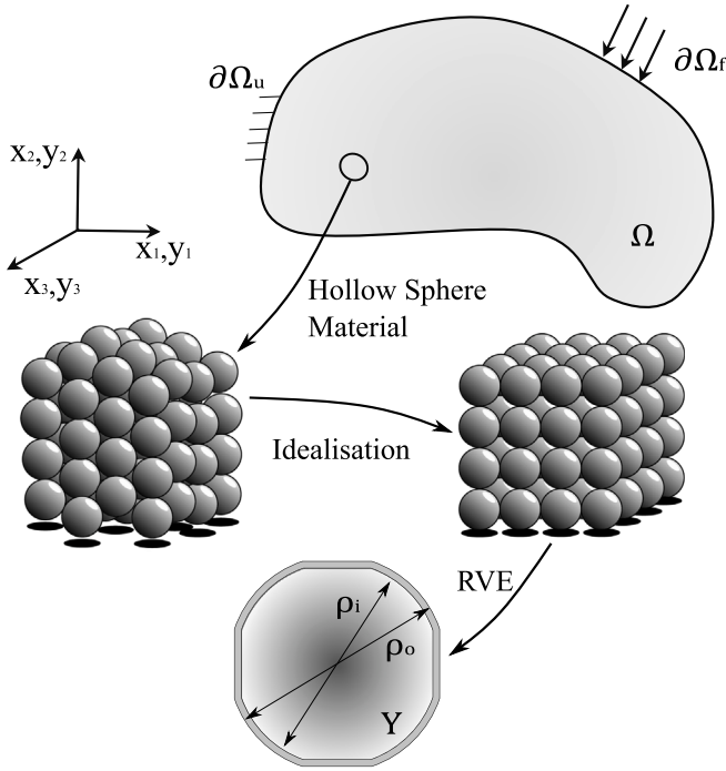
Fig. 1. Depiction of the microscopic structure of a small portion of the macroscopic domain, idealised model and the RVE.
