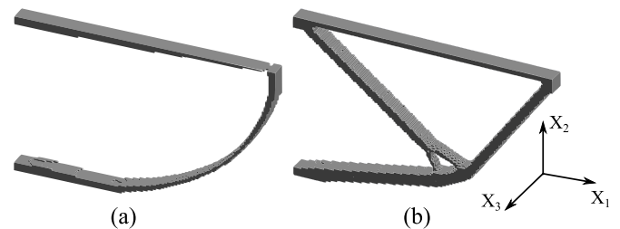
Fig. 9. Qualitative comparison for case cb_2 between the optimised distribution of relative densities for cases (a) \bar{V} = 5\% and (b) the optimum distribution of material using SIMP.
