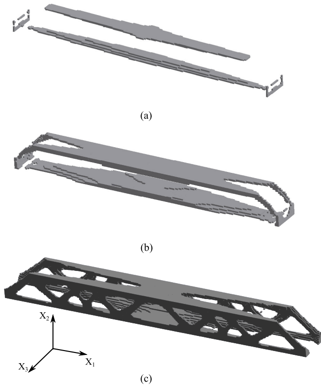
Fig. 10. Qualitative comparison for case 3pb_1 between the optimised distribution of relative densities for (a) \bar{V} = 5\% , (b) \bar{V} = 10\% , and (c) the optimal distribution of material using SIMP.
