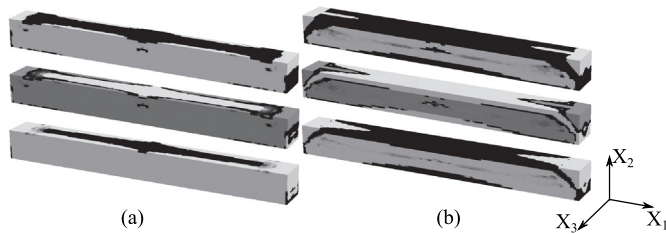
Fig. 7. Optimum distribution of hollow spheres for the case 3pb_1. External diameter, internal diameter and relative density for cases with (a) \bar{V} = 5\% , and (b) \bar{V} = 10\% . A linear scale is considered between the minimum admissible value (light grey) and the maximum admissible value (black) for the considered variables.
