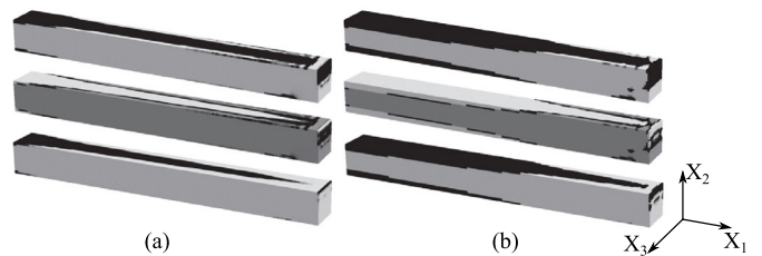
Fig. 6. Optimum distribution of hollow spheres for the case cb_1. External diameter, internal diameter and relative density for cases with (a) \bar{V} = 5\% , and (b) \bar{V} = 10\% . A linear scale is assumed between the minimum admissible value (light grey) and the maximum admissible value (black) for the considered variables.
