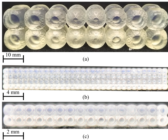
Fig. 13. Variation on the size and number of hollow spheres. The structures were printed with (a) 16, (b) 512, and (c) 128 spheres.
