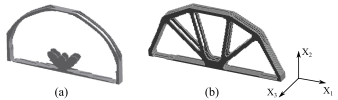
Fig. 11. Qualitative comparison for case 3pb_2 between the optimised distribution of relative densities for (a) \bar{V} = 5\% and (b) the optimum distribution of material using SIMP.
