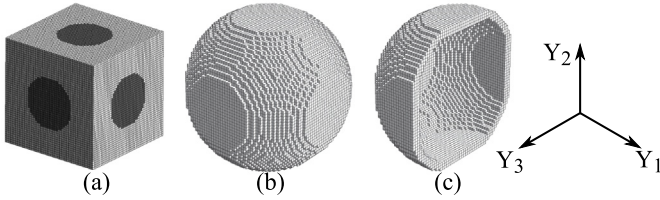
Fig. 4. The FE mesh for the hollow sphere model: (a) complete FE mesh; FE mesh with void elements suppressed for (b) the entire RVE and (c) a cross-section of the RVE.
