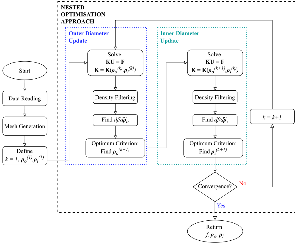
Fig. 3. Flowchart of the optimisation framework depicting the update of outer and inner diameters.
