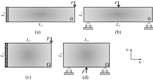
Fig. 2. Design domains considered for the optimisation problem: (a) cantilever beam (cb_1), (b) 3-point bending beam with load application on the upper side (3pb_1), (c) cantilever beam (cb_2), and (d) 3-point bending beam with load application on the bottom side (3pb_2).
