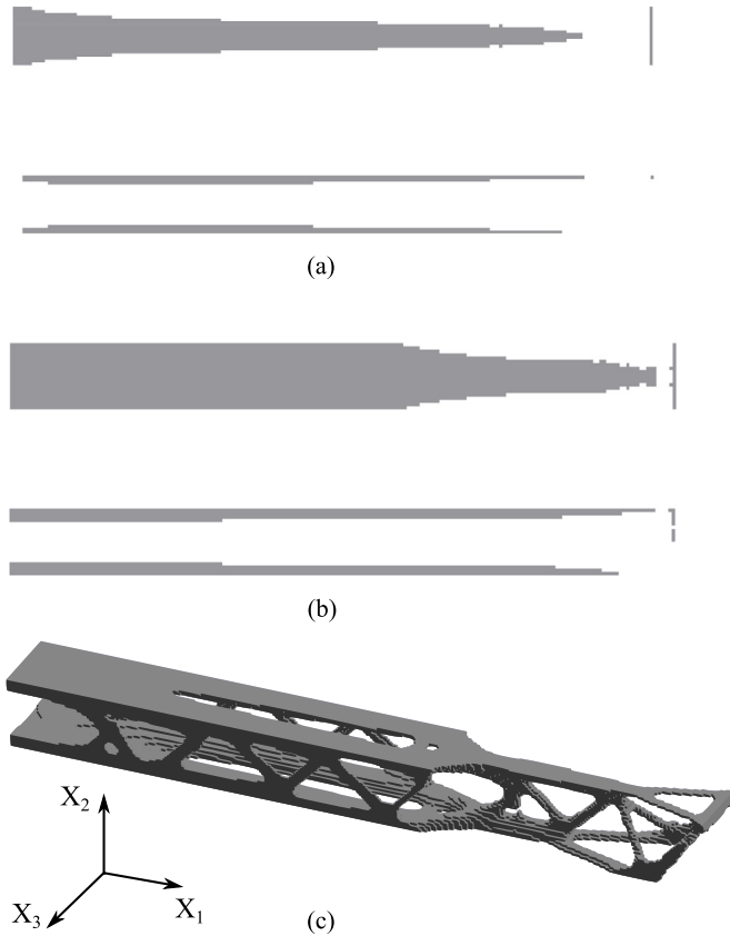
Fig. 8. Qualitative comparison for case cb_1 between the optimised distribution of relative densities for (a) \bar{V} = 5\% , (b) \bar{V} = 10\% , and (c) the optimum distribution of material using SIMP.
