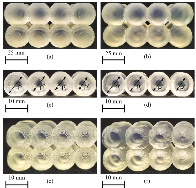
Fig. 12. Variation of geometrical parameters of the printed hollow sphere structures. Homogeneous distribution with (a) non-smooth geometry and (b) smooth geometry. Variation of the internal diameter for (c) non-smooth geometry, and (d) smooth geometry. Variation of the external diameter for (e) non-smooth geometry, and (f) smooth geometry.
