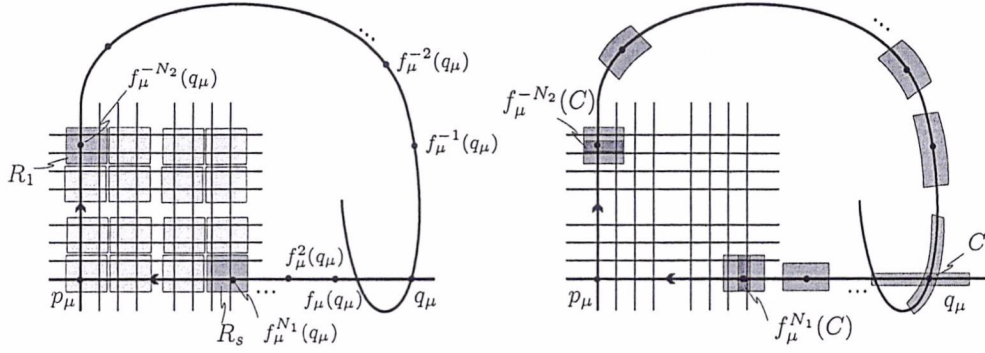
FIGURE 2. Construction of the Markov partition.
