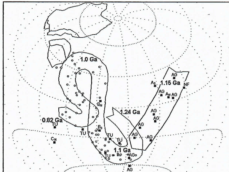
Figure 2. Configuration of Amazonian Craton and Laurentia, as presented in D'Agrella-Filho et al. (1998) (Laurentia is in its present position). The present paleomagnetic data for the Amazonian Craton (full squares) is compared with the APW path for Laurentia (empty circles) in the time interval: 1.24-0.82 Ga. AG: VGPs from the Aguapeí sediments; TU: VGPs from crystalline basement rocks (Rio Negro-Juruena Province); NF: paleomagnetic pole for the Nova Floresta Formation; A S , A N , B S , B N and C N : paleomagnetic poles from the Nova Brasilândia Group and the Serra da Providência Intrusive Suite.
