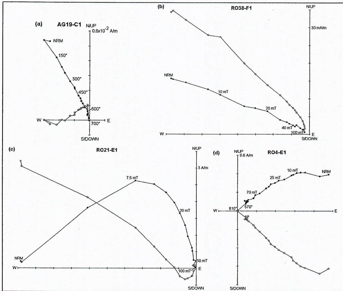
Figure 1. Examples of AF and thermal demagnetizations. Zijderveld projections: full (empty) symbols represent horizontal (vertical) projections (see text for details).
