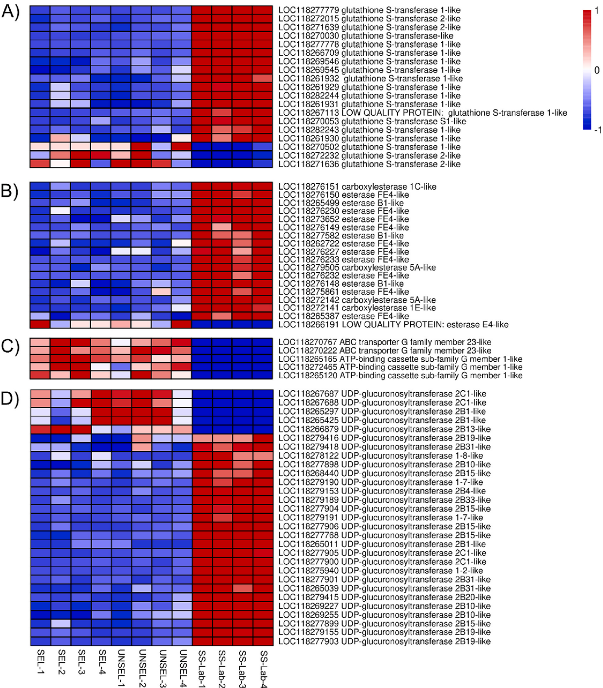
Fig. 4. Heatmap of the expression of A) Glutathione-S-transferases, B) esterases, C) ABC transporters and D) UDP-glycosyltransferases genes in susceptible (SS-Lab), Selected (Sel) and Unselected (Unsel) strains of Spodoptera frugiperda .
