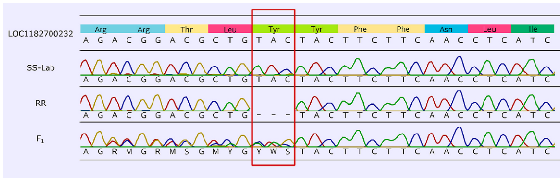
Fig. 5. Representative chromatograms from Sanger sequencing of the nAChR α6 PCR product from individuals of the susceptible (SS-Lab), spinetoram-resistant (RR) and F 1 crosses of these strains. The location of the Y232del is indicated with a red box. (For interpretation of the references to colour in this figure legend, the reader is referred to the web version of this article.)
