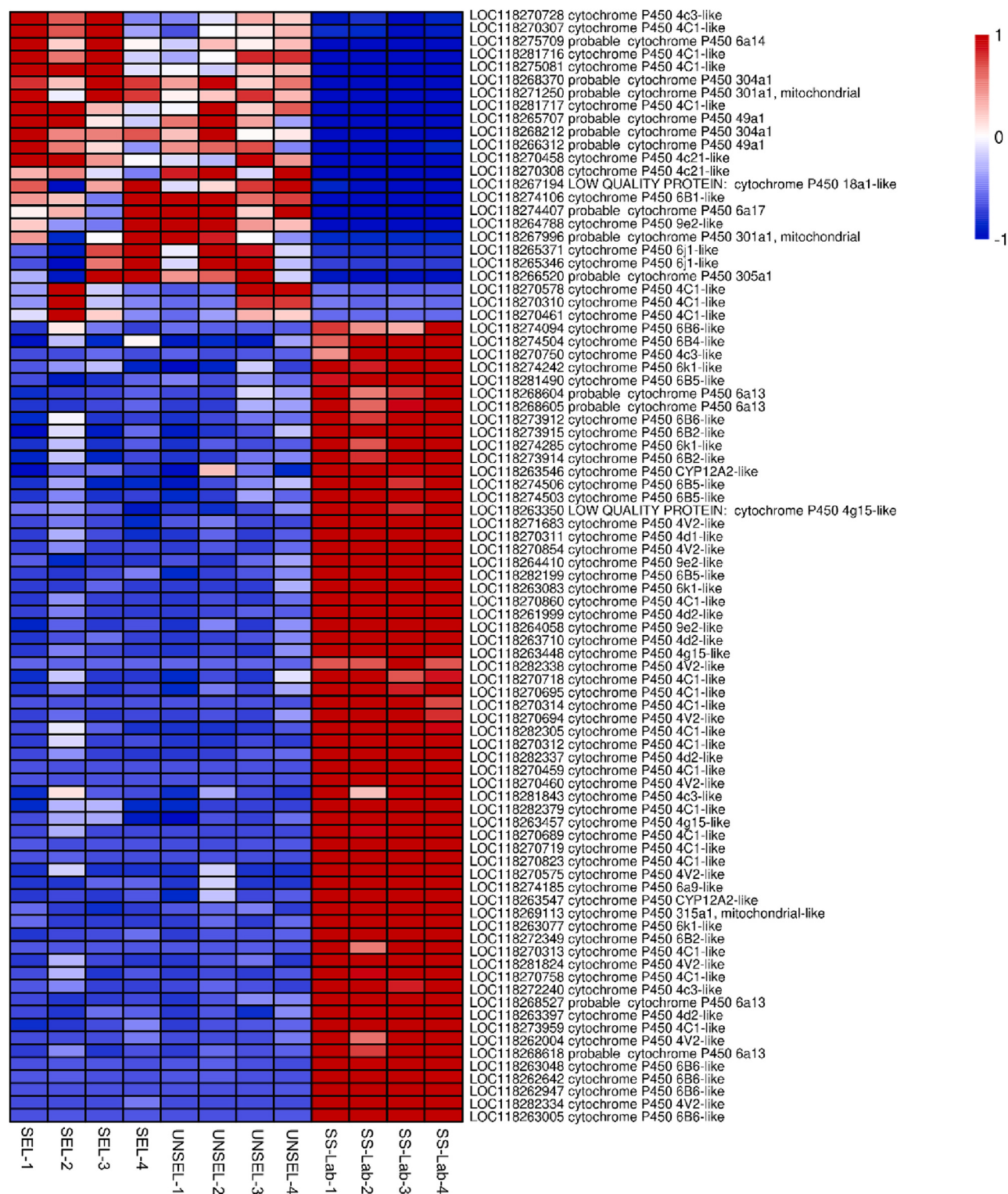
Fig. 3. Heatmap of the expression of cytochrome P450 genes in the susceptible (SS-Lab), Selected (Sel) and Unselected (Unsel) strains of Spodoptera frugiperda .
