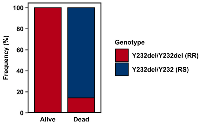
Fig. 6. Frequency of the Y232del mutation in alive and dead Spodoptera frugiperda individual larvae following exposure to a discriminating concentration of spinetoram. n dead = 21, n alive = 21. A significant association was observed between the insect genotype and its phenotype by chi-square test ( \chi^2 = 28.1 , df = 1 , p < 0.001 ).
