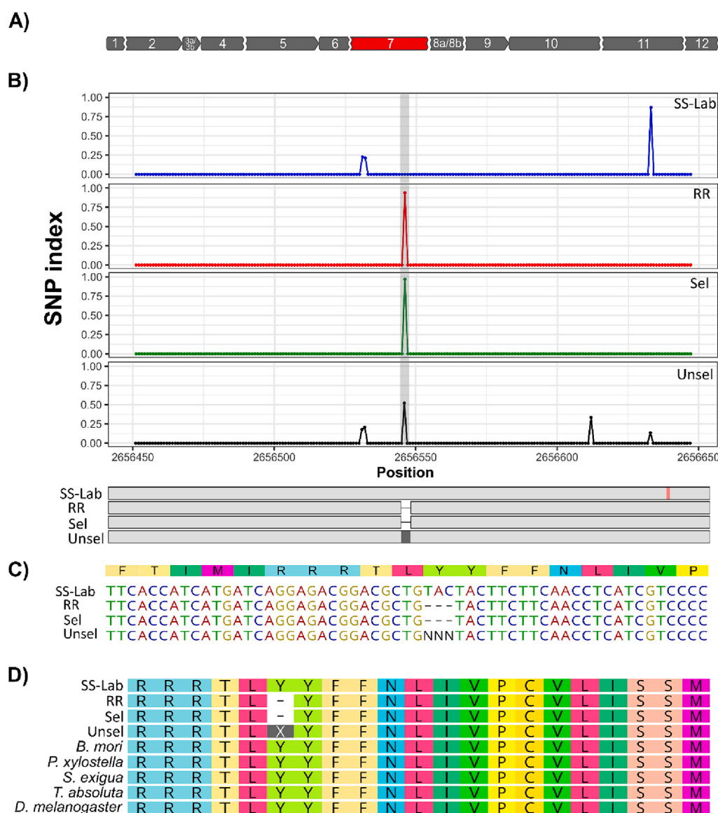
Fig. 1. Characterization of a three nucleotide deletion in the nAChR \alpha 6 gene of Spodoptera frugiperda associated with spinetoram resistance. A) Exon structure of the nAChR \alpha 6 gene highlighting exon 7 where a mutation was identified. B) SNP index in exon 7 of the nAChR \alpha 6 gene for the SS-Lab, RR, Sel and Unsel strains. C) A triplet deletion presented in RR and Sel strains results in the deletion of an amino acid (Y232del). D) Alignment of the amino acids sequences of nAChR \alpha 6 from other insect species. The accession numbers of the shown sequences are: Bombyx mori (NP_001091842.2), Plutella xylostella (ADD69773.1), Spodoptera exigua (QIC53910.1), Tuta absoluta (ALM23508.1) and Drosophila melanogaster (NP_723494.2).
