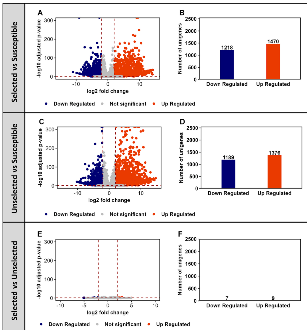
Fig. 2. Differentially expressed gene (DEG) analysis in comparisons of the susceptible (SS-Lab), Selected (Sel) and Unselected (Unsel) strains of Spodoptera frugiperda . A) Volcano plot of the DEGs for Sel vs SS-Lab; B) Number of up- and down-regulated DEGs for Sel vs SS-Lab; C) Volcano plot of the DEGs for Unsel vs SS-Lab; D) Number of up- and down-regulated DEGs for Unsel vs SS-Lab; E) Volcano plot of the DEGs for Sel vs Unsel; F) Number of up- and down-regulated DEGs for Sel vs Unsel.
