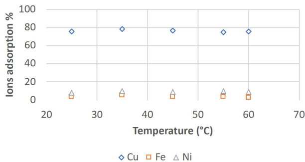
Figure 7. Percentage ions adsorbed varying the temperature in 120min, 1g of resin, pH 1.5 and 50mL of solution.
