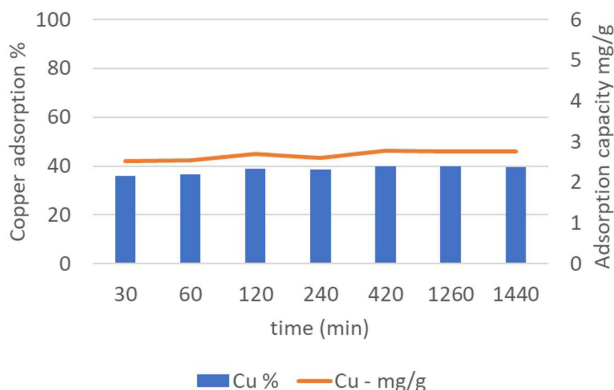
Figure 2. Percentage of copper ions adsorbed and adsorption capacity (mg/g) during the time (30-1440min) using 1g of resin, 50mL of solution and pH 0.5 at 25°C.
