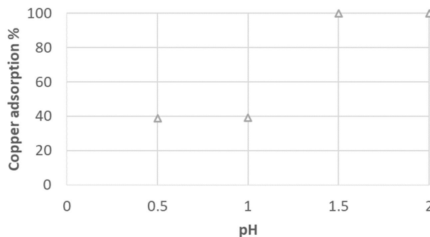
Figure 3. Percentage copper adsorbed for each pH studied in 120min, using 1g of resin, 50mL of solution at 25°C. Δ = Percentage of copper ions adsorption.
