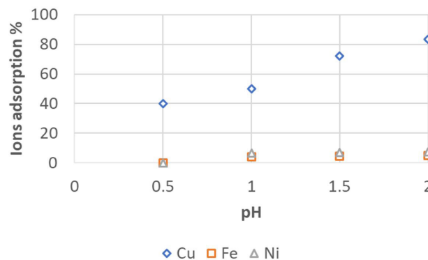
Figure 5. Percentage ions adsorbed for each pH studied in 120min, using 1g of resin, 50mL of solution at 25°C.
