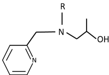
Figure 1. The hydroxypropyl-picolylamine functional group of Dowex XUS 43605 chelating resin [12].
