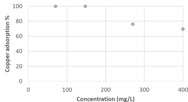
Figure 4. The effect of copper concentration in 120min, at pH 1.5, using 1g of resin and 50mL of solution at 25°C. ◇ = Percentage of copper ions adsorption.
