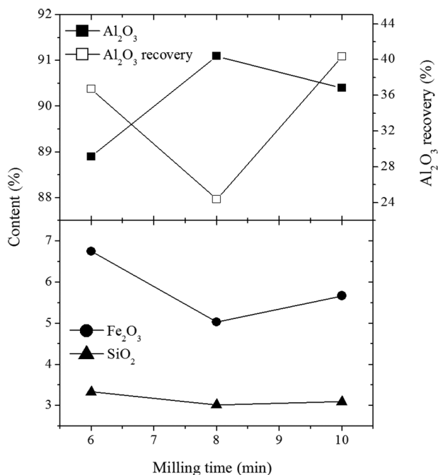
Figure 4. Influence of the milling time on the gibbsite flotation performance.
