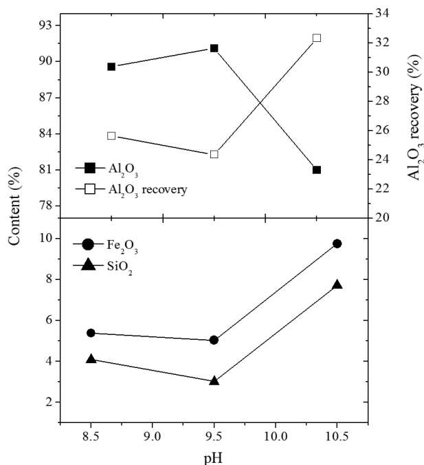
Figure 3. Influence of pH on the gibbsite flotation.
