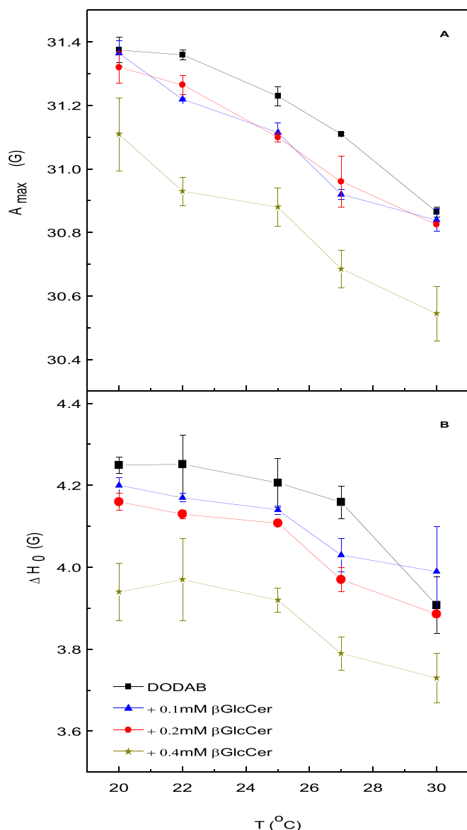
Fig. 4. Effect of \beta GlcCer on the maximum hyperfine splitting ( A_{max} ) of 5-PCSL (A) and on the central field linewidth ( \Delta H_0 ) of 16-PCSL (B) embedded in 2 mM DODAB bilayers at the gel phase.
