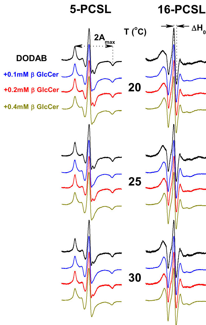
Fig. 3. Effect of \beta GlcCer on ESR spectra of 5-PCSL and 16-PCSL embedded in 2 mM DODAB bilayers at temperatures below the gel-fluid transition. The maximum hyperfine splitting ( A_{\max} ) and the central field linewidth ( \Delta H_0 ) are indicated. Total spectra width is 100 G.
