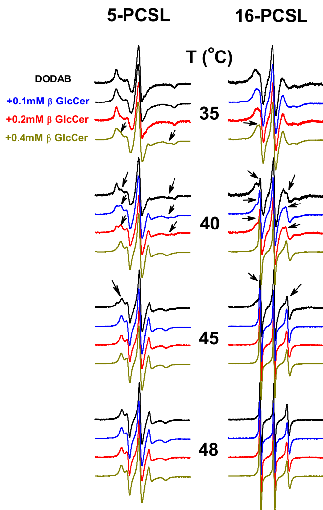
Fig. 5. ESR spectra of 5-PCSL and 16-PCSL embedded in 2 mM DODAB or 2 mM DODAB + \beta GlcCer bilayers around the gel-fluid transition. Arrows indicate features of a more isotropic component which coexists with the typical gel phase signal.
