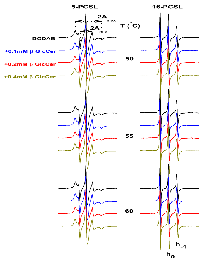
Fig. 6. Effect of \beta GlcCer on ESR spectra of 5-PCSL and 16-PCSL embedded in 2 mM DODAB bilayers at temperatures above the gel-fluid transition. Maximum and minimum hyperfine splittings ( A_{max} and A_{min} ) are indicated, as well as the positions of central ( h_0 ) and high ( h_{-1} ) field lines. Total spectra width is 100 G.
