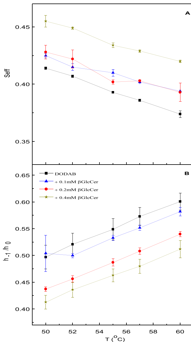
Fig. 7. Effect of mM \beta GlcCer on the effective order parameter ( S_{eff} ) from 5-PCSL spectra (A) and on h_{-1}/h_0 ratios from 16-PCSL spectra (B) embedded in 2 mM DODAB bilayers at the fluid phase.
