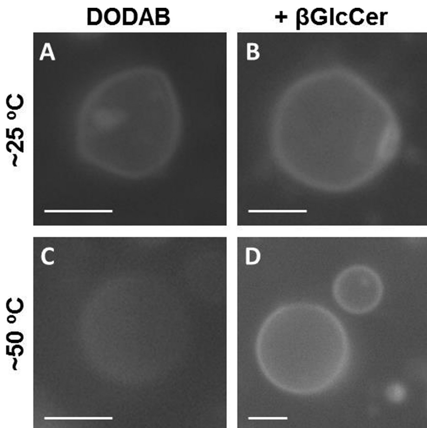
Fig. 8. Fluorescence microscopy (0.5 mol% PE-Rh) images of vesicles of 2 mM DODAB (A and C) and 2 mM DODAB + 0.2 mM \beta GlcCer (B and D) in the gel (A and B) and fluid (C and D) phases. The scale bar represents 4 \mu m. The image in C was obtained after long exposure of the vesicle to the illumination, which caused significant fluorescence photobleaching. The contrast of the snapshots was enhanced.
