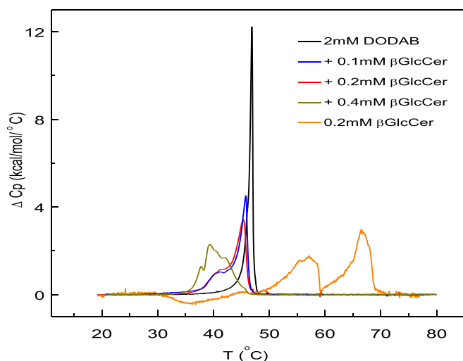
Fig. 2. Effect of \beta GlcCer on the DSC thermogram of 2 mM DODAB bilayers. Scan rate was 5 °C/h.
