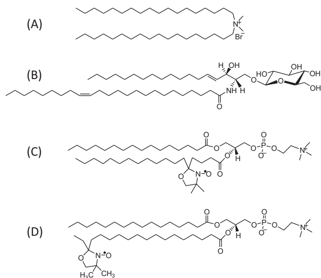
Fig. 1. Chemical structures of DODAB (A), βGlcCer (B), 5-PCSL (C) and 16-PCSL (D).
