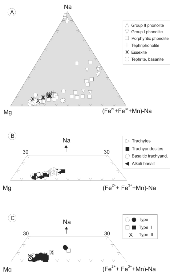
Figure 4. A: Clinopyroxenes of rocks of the Remédios sodic series showing the increase in Na (and decrease in Mg, Fe_{total} and Mn) in more differentiated rocks. B: Clinopyroxene compositions in rocks of the Remédios moderately potassic series showing a slight increase in Na with differentiation. C: Clinopyroxenes in Remédios lamprophyres. Source: [1, 2, 13].
