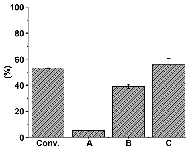
Figure 4. Conversion of cyclohexene (%) and product selectivity (%) (A = 1,2-epoxycyclohexane; B = cyclohexen-1-one; C = 2-cyclohexen-1-ol) when using ND@βNH-TPPpCF 3 -Cu(II) as catalyst.
