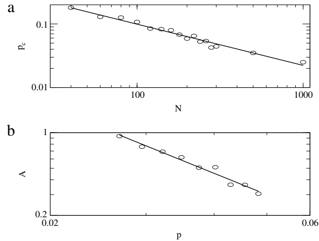
Fig. 5. (a) Critical probability of shortcuts as a function of network size; (b) amplification factor as a function of the shortcut probability. The full lines are least-squares fits. The time delay is zero and the remaining network parameters are the same as in the previous figures.
