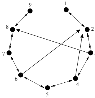
Fig. 1. Schematic representation of a small-world network of the Newman–Watts time with N = 9 nodes and free boundary conditions.
