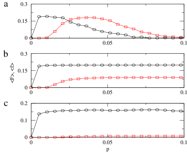
Fig. 4. (Color online) Average firing rate per neuron ( \langle F \rangle ) (black circles) and average firing rate per neuron ( \langle f \rangle ) for nonlocal connections only (red squares) as a function of the shortcut probability p , for 200 different realizations of the connectivity matrix and 1000 time instants. We considered a cellular automata with N = 100 , \mu = 5 , and: (a) \tau = 0 , (b) \tau = 10 and (c) \tau = 100 .
