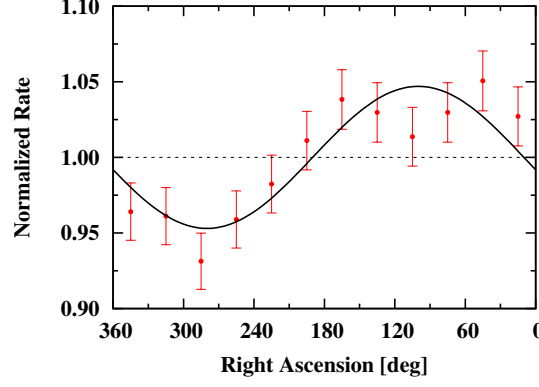
Figure 1: Observed number of events, normalized to the mean, as a function of the right ascension, for E \geq 8 EeV. The black line is a sinusoidal function showing the first harmonic from Table 1.
