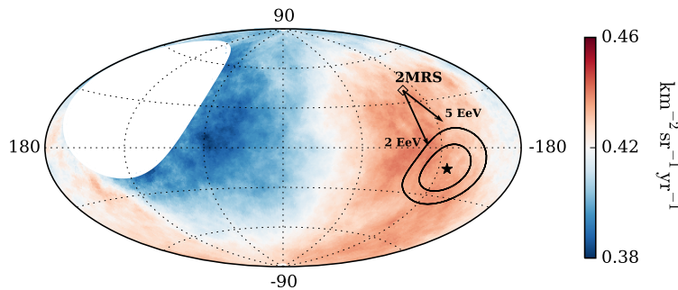
Figure 3: Map of the flux in Galactic coordinates for E \geq 8 EeV, smoothed on windows of 45^\circ . The reconstructed dipole direction is indicated with a star, the contours represent the 68% and 95% CL regions. Also indicated is the direction of the dipole in the distribution of galaxies from 2MRS and how a dipole along this direction would be modified by the action of the Galactic magnetic field.
