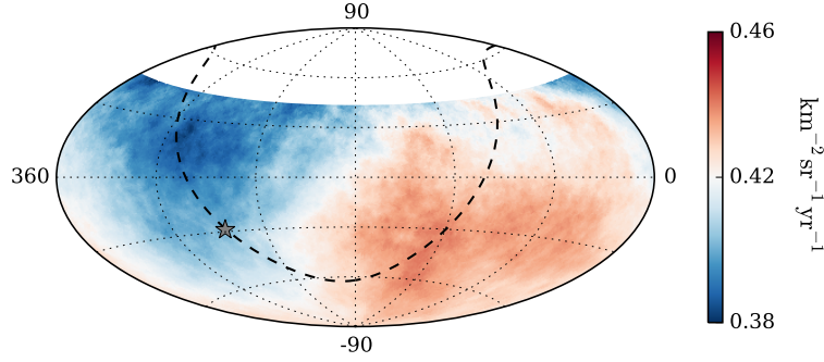
Figure 2: Map of the flux of cosmic rays above 8 EeV in equatorial coordinates and smoothed with a 45^\circ top-hat window. The star represents the direction of the Galactic center and the dashed line shows the Galactic plane.
