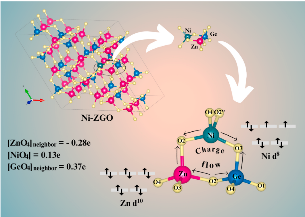
Fig. 7. Schematic representation of the [NO 4 ], neighbor [ZnO 4 ] (at the six-membered rings composed only by Zn2 sites) and [GeO 4 ] (at the six-membered rings composed by Z1 sites and Ge). Values of the Mulliken charges and the respective metal electronic configuration induced by the Ni 2+ -doping process.
