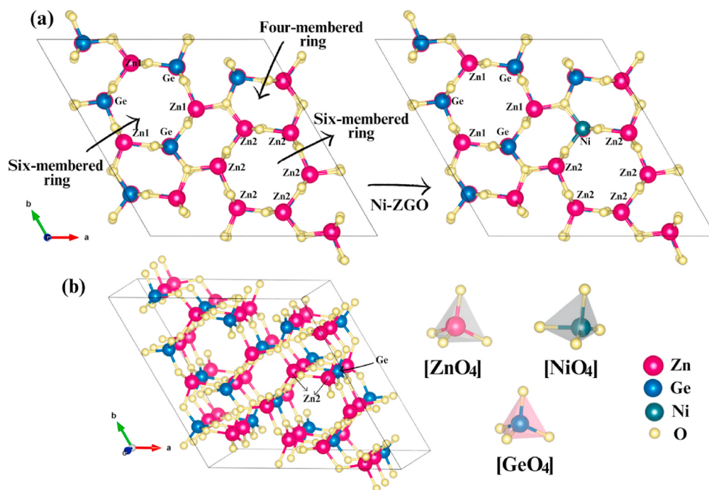
Fig. 1. (a) ZGO structure is composed of the six- and four-membered rings involving the [ZnO 4 ] and [GeO 4 ] clusters. The most energetically favorable Ni 2+ -doping process occurs at the Zn2 site. (b) 3D view of the ZGO structure and the [ZnO 4 ], [NiO 4 ], and [GeO 4 ] clusters.
