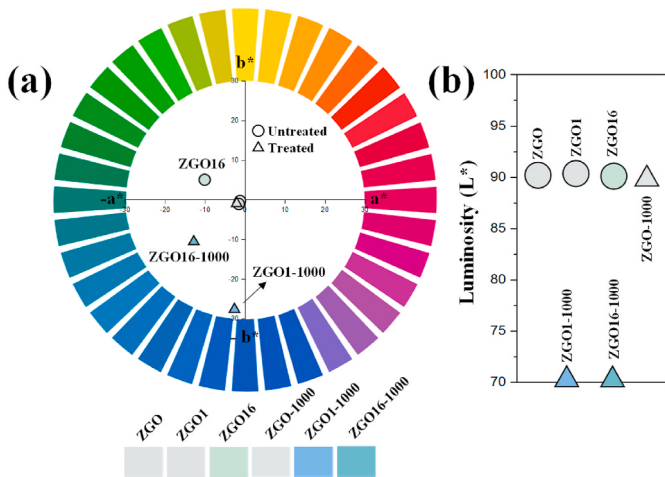
Fig. 9. (a) a^* (green and red), b^* (yellow and blue) and (b) L^* (lightness, with 100 representing white and 0 representing black) CIE Lab coordinates for the samples. (For interpretation of the references to color in this figure legend, the reader is referred to the Web version of this article.)
