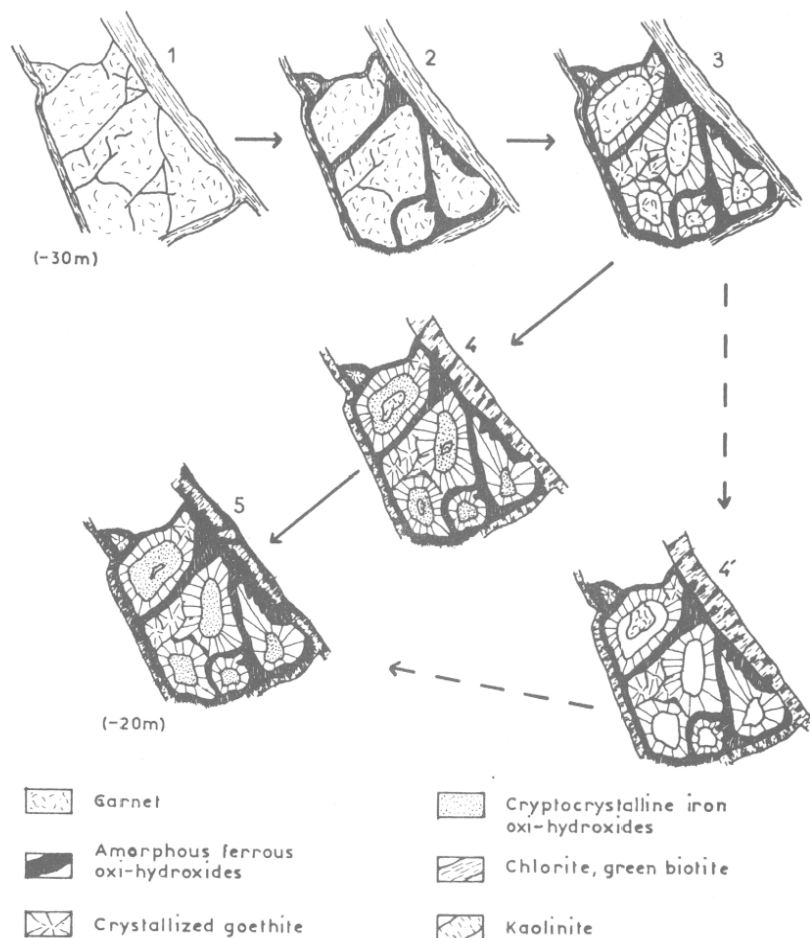
Fig. 1 : Schematic representation of garnet weathering
