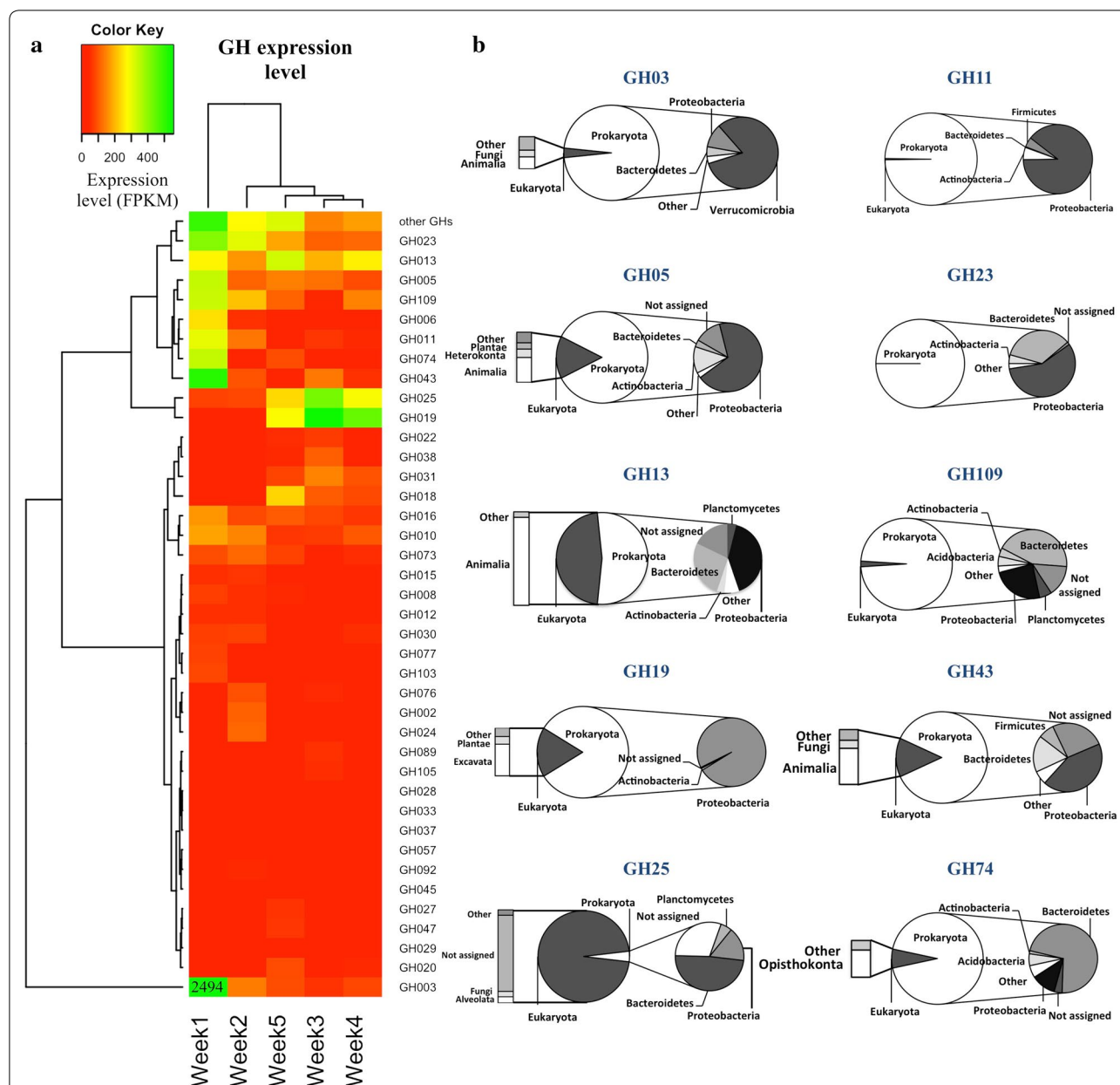
Fig. 5 Differential expression and phylogenetic distribution of glycoside hydrolase (GH) families identified in sugarcane bagasse composting community metatranscriptome. a Heat map representation of the GHs expression. Columns represent time when sample was collected. Rows depict different GHs families identified in the metatranscriptome dataset. The color key for GH 3 expression at week 1 is out of range with expression level of 2494. GH families were grouped based on substrate preferences, as reported elsewhere [93]. b Phylogenetic assignment of reads belonging to the most expressed families using the Lowest Common Ancestor algorithm
