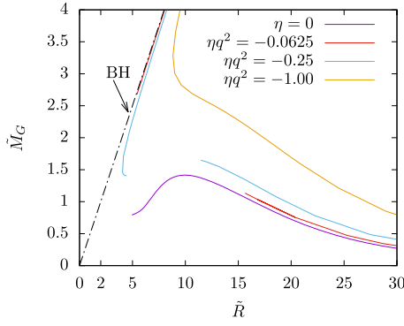
Fig. 7. We show the mass \tilde{M}_G as function of the radius \tilde{R} of the neutron star solutions for \Gamma = 3/5 (left) and \Gamma = 2.34 (right) for several values of \eta q^2 . The mass-radius relation of the corresponding Schwarzschild black hole is indicated by “BH”.
