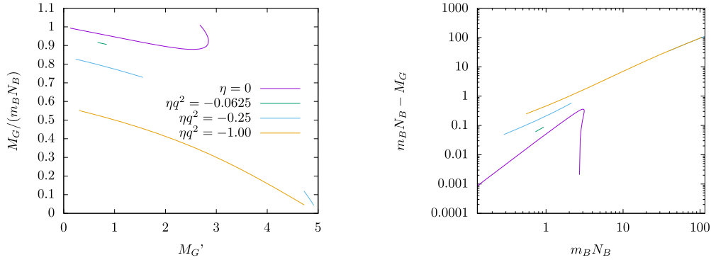
Fig. 10. Left: We show the ratio M_G/(m_B N_B) between the mass M_G of the neutron star and the mass of N_B individual baryons of mass m_B in function of M_G for EOSIII and several values of \eta q^2 . Right: We show the difference in energy between N_B baryons of mass m_B and the mass M_G of the neutron star in function of m_B N_B .
