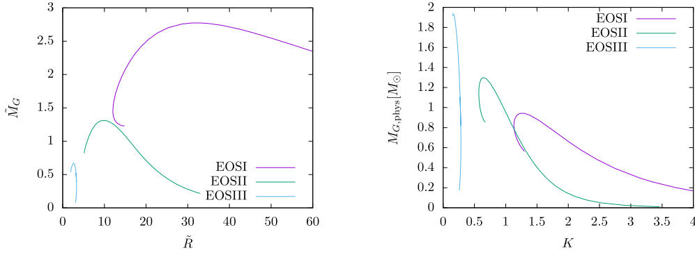
Fig. 5. We show the mass \tilde{M}_G as function of the radius \tilde{R} of the neutron star solutions for \eta = 0 and three different EOS, see (29), respectively (left). We also show M_{G,phys} in units of solar masses M_\odot as function of K for the same EOS and R = 10 (right).
