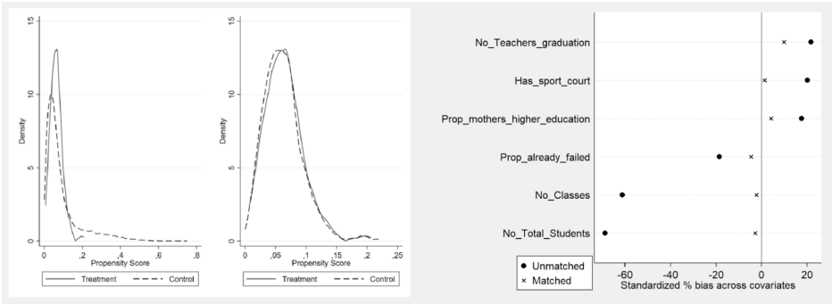
(a) Common Support (b) Covariates Balance
