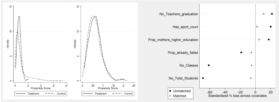
(a) Suporte Comum (b) Covariates Balance
